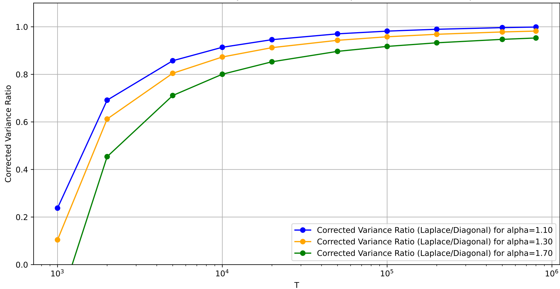
Corrected Variance Ratio Trajectories for Different Alphas, \text{dim}=(Tb50)^{**}(1b\alpha)
