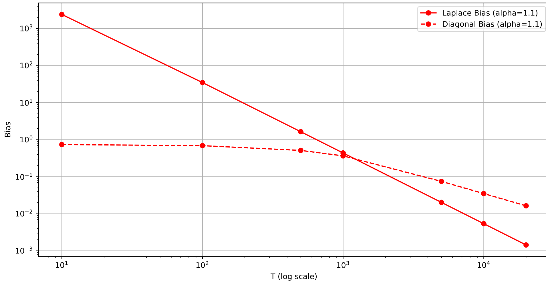
Bias Trajectories for Different Alphas (Laplace vs Diagonal) for Linear schedule
