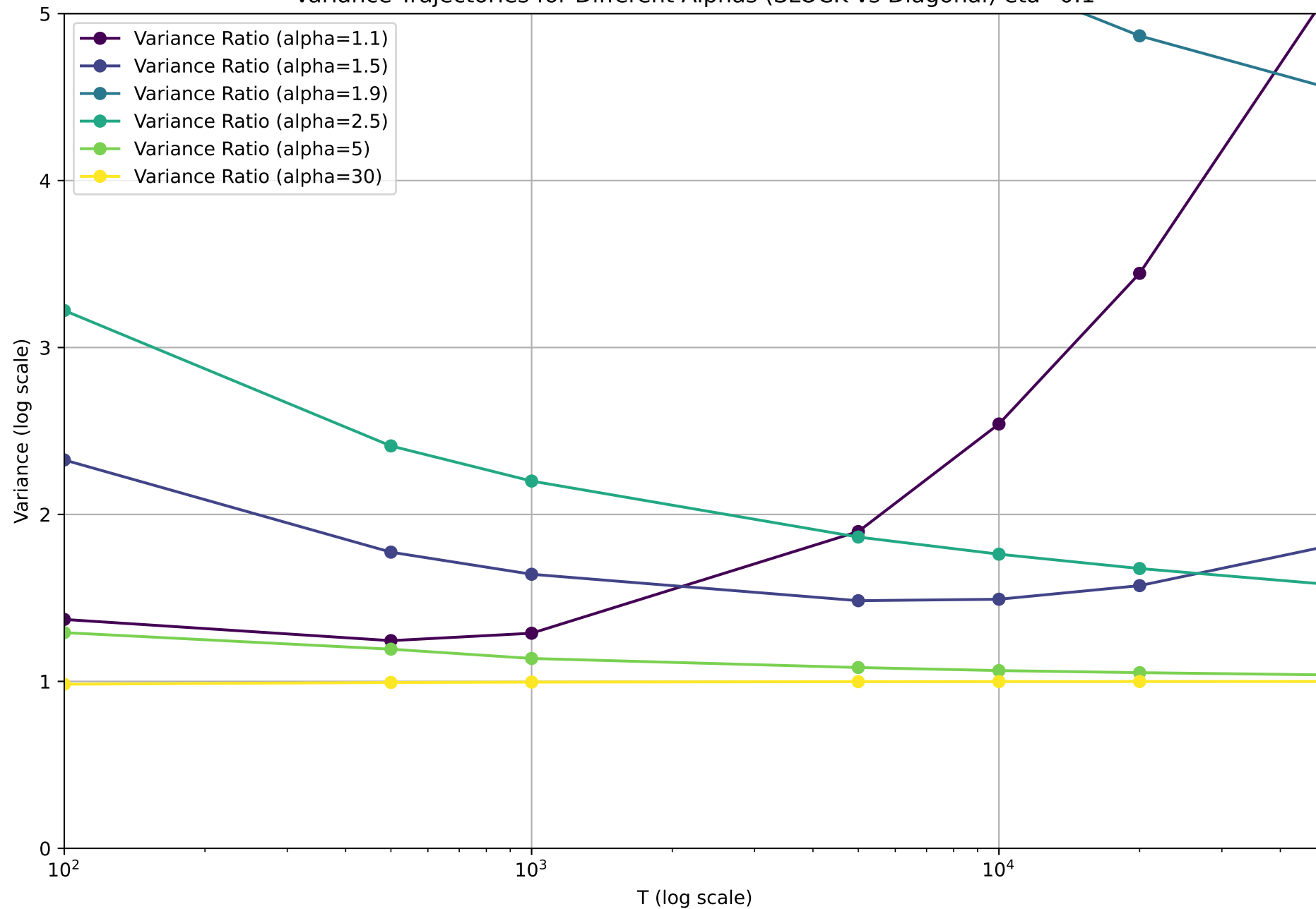
Variance Trajectories for Different Alphas (SLOCK vs Diagonal) \eta=0.1
