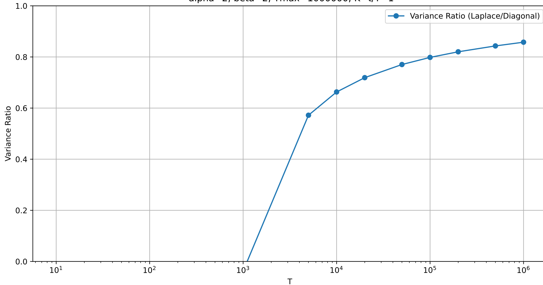
Variance Ratio of Laplace approximation to Diagonal approximation for linear schedule \alpha=2 , \beta=2 , T_{\max}=1000000 , K=t/T=1
