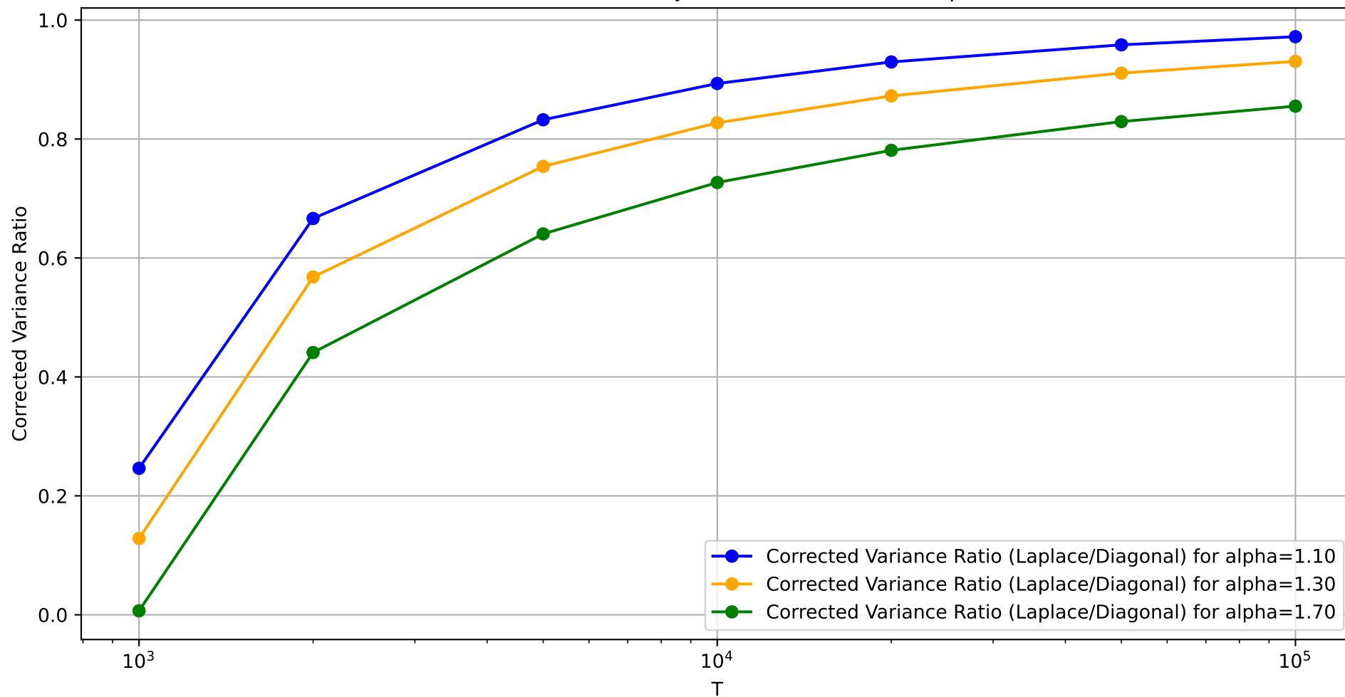
Corrected Variance Ratio Trajectories for Different Alphas, 0.01T
