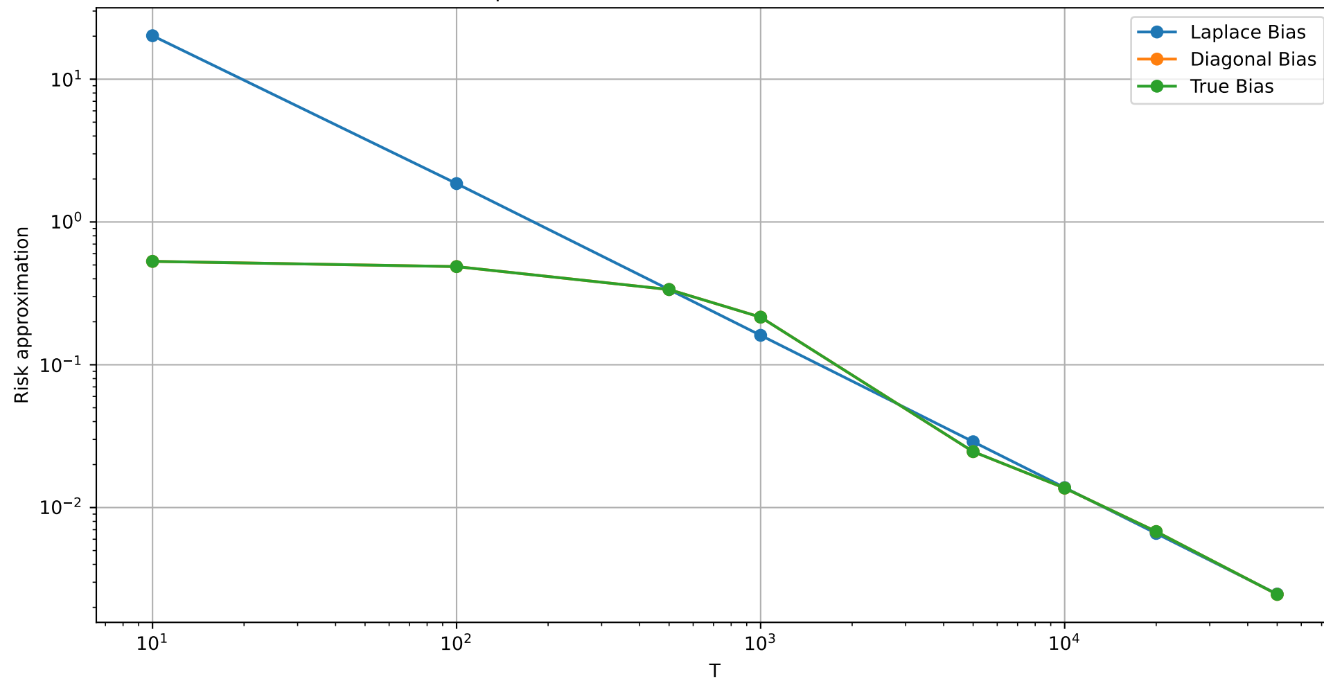
Bias components of Laplace approximation vs Diagonal approximation for linear schedule \alpha=3 , \beta=1.2 , T_{\max}=50000 , K=t/T=1
