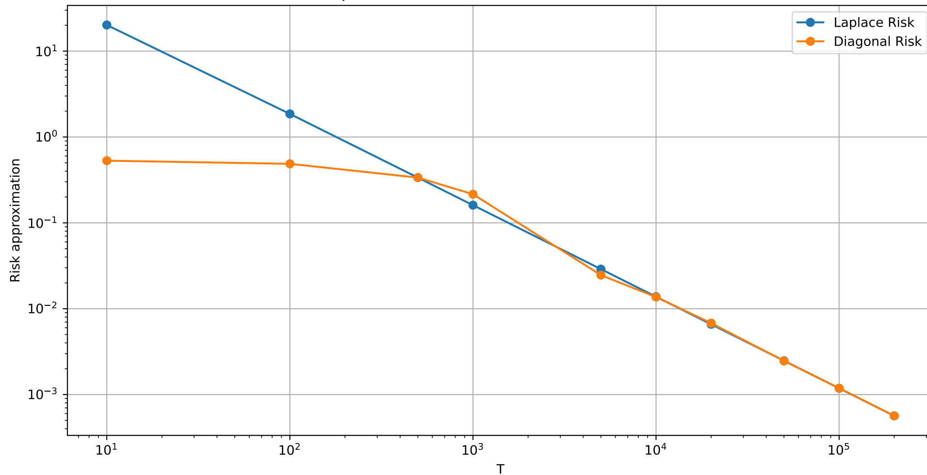
Total risk of Laplace approximation vs Diagonal approximation for linear schedule \alpha=3 , \beta=1.2 , T_{\max}=200000 , K=t/T=1
