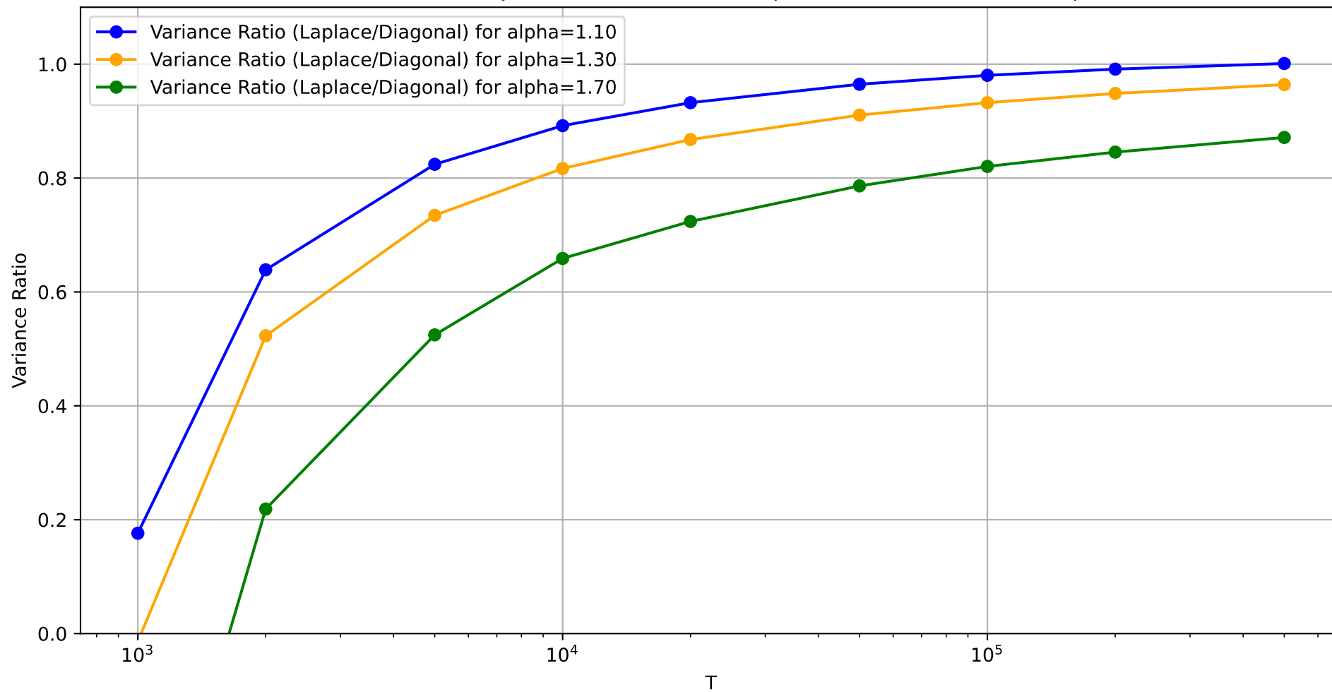
Variance Ratio Trajectories for Different Alphas, \text{dim}=(Tb100)^{*(1/\alpha)}
