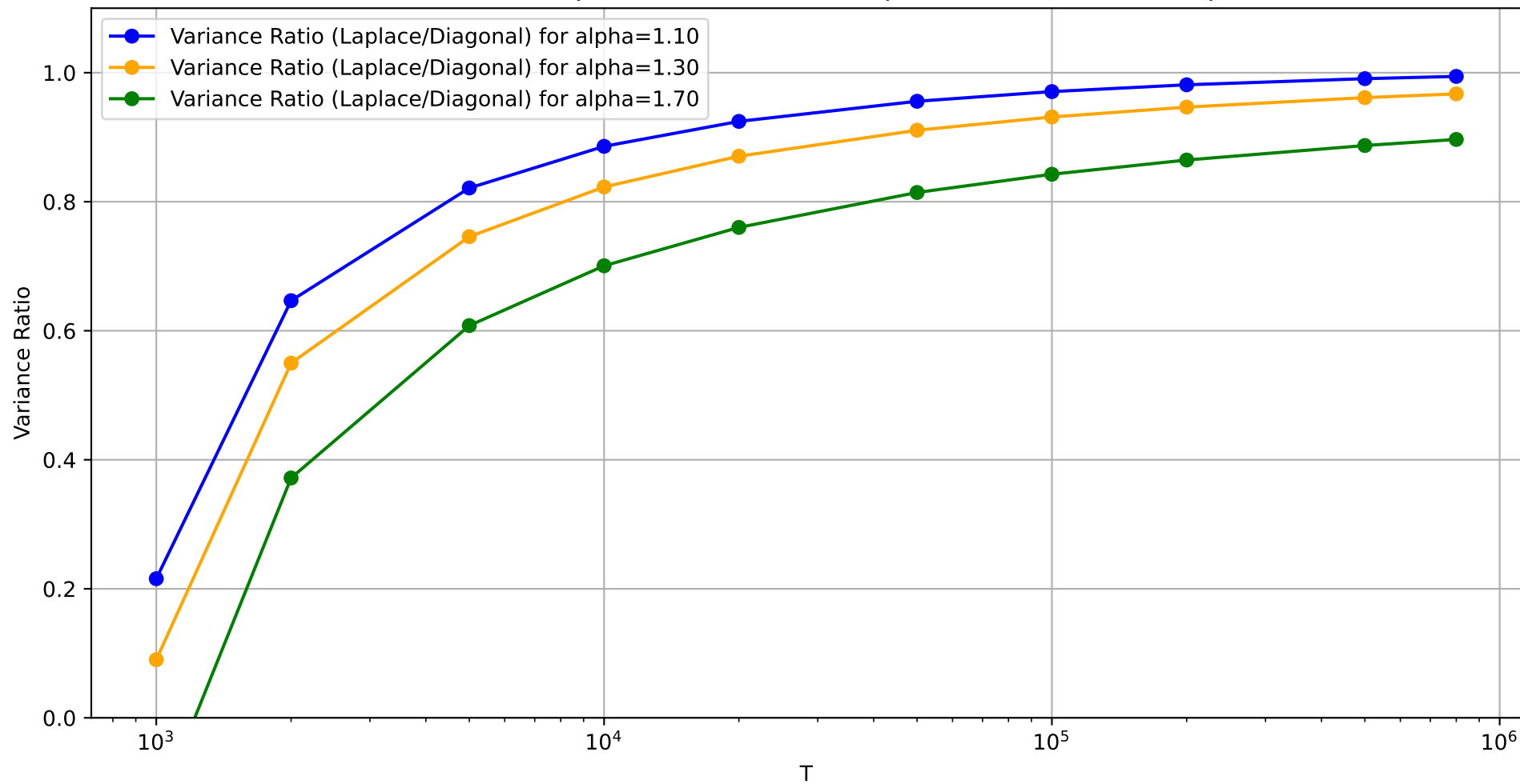
Variance Ratio Trajectories for Different Alphas, \text{dim}=(\text{Tb50})^{**}(1/\alpha)
