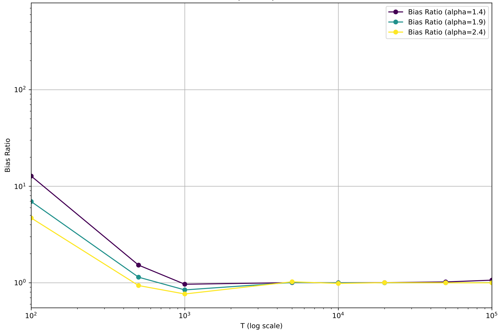
Bias Ratios for Different Alphas (equivalent vs exact) \eta=0.001
