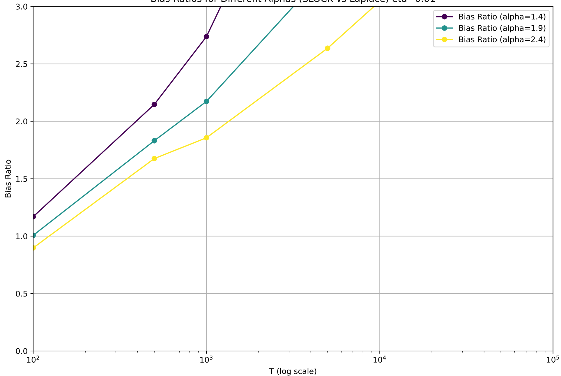
Bias Ratios for Different Alphas (SLOCK vs Laplace) \eta=0.01
