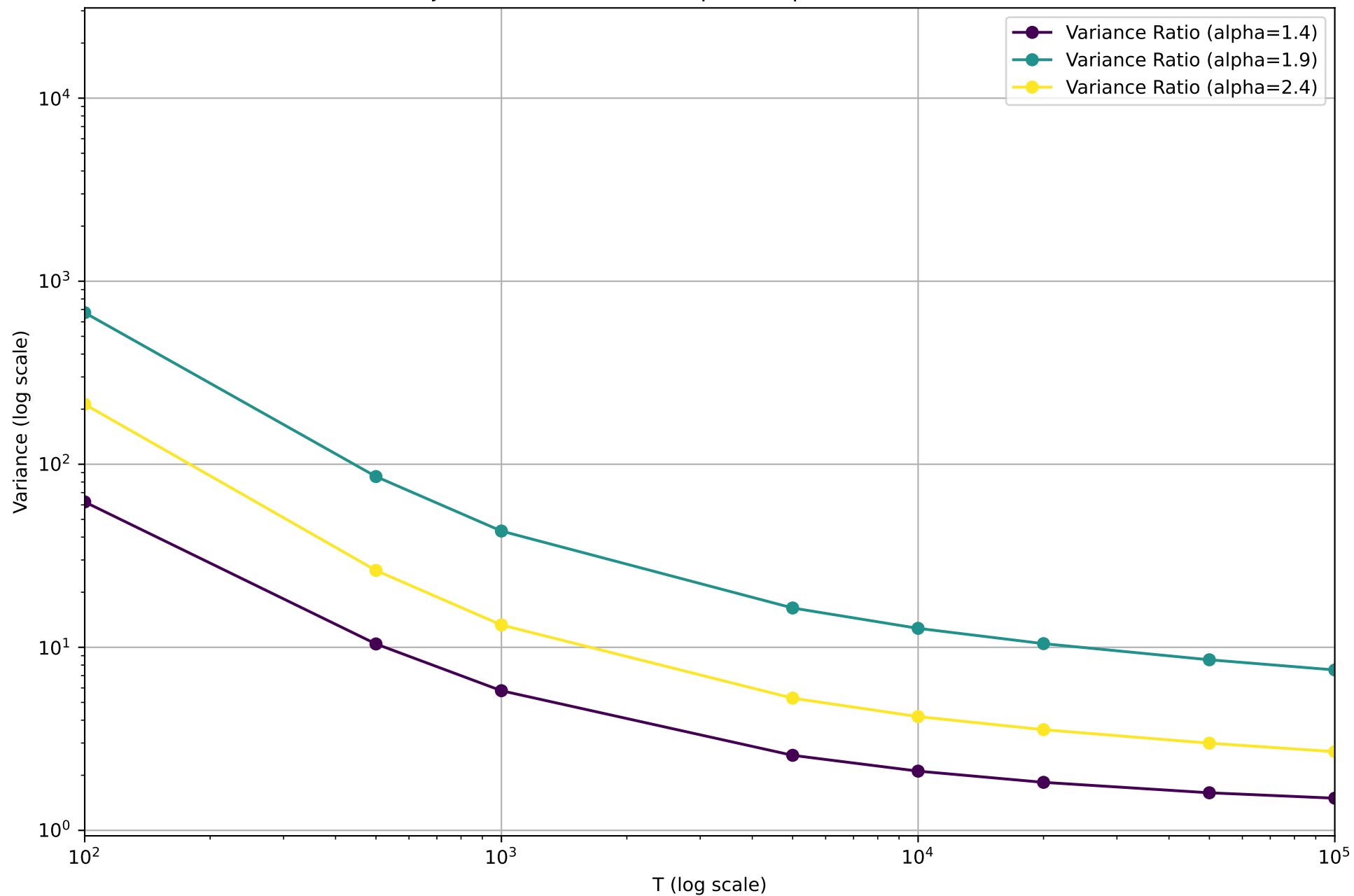
Variance Trajectories for Different Alphas (equivalent vs exact) eta=0.001
