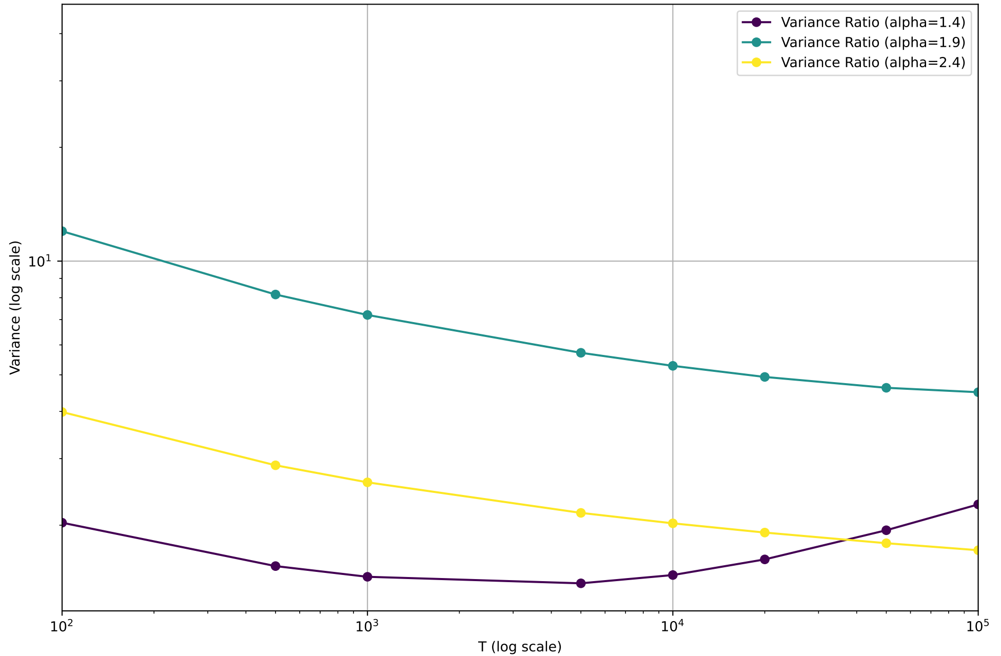
Variance Trajectories for Different Alphas (equivalent vs exact) \eta=0.1
