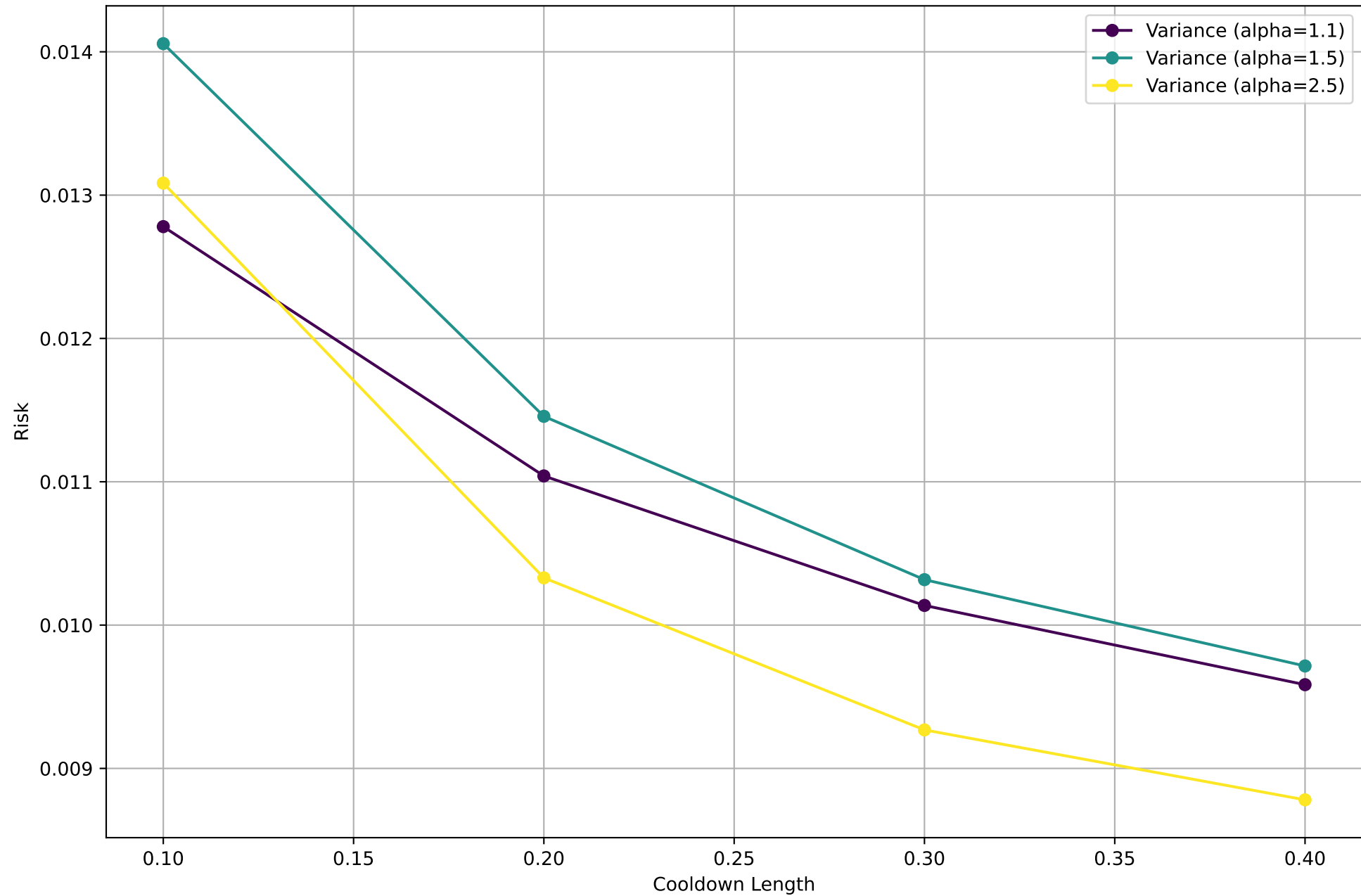
Risk for Different Alphas (SLOCK vs Diagonal) \eta=0.01 , T=1000
