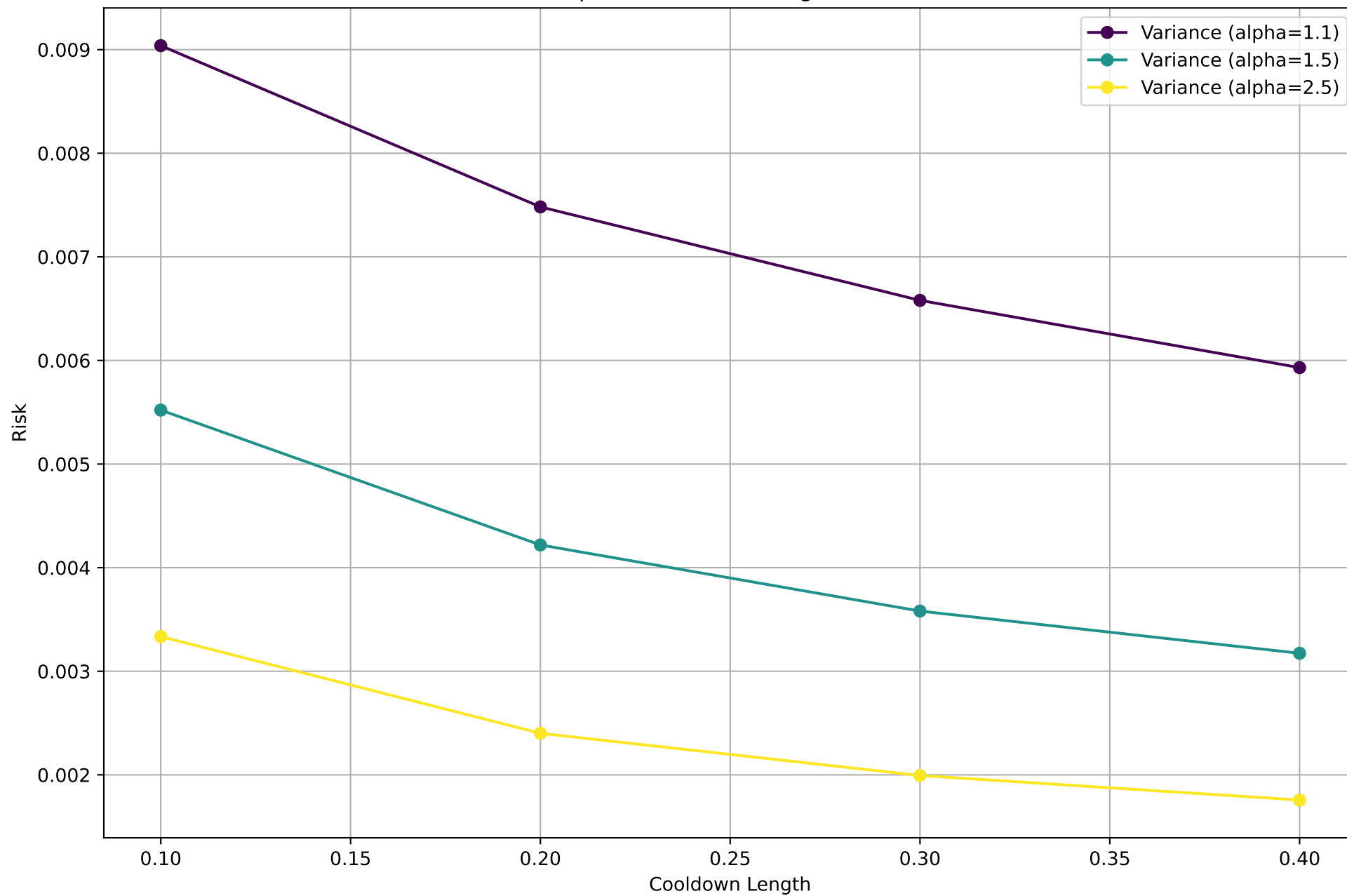
Risk for Different Alphas (SLOCK vs Diagonal) \eta=0.01 , T=10000
