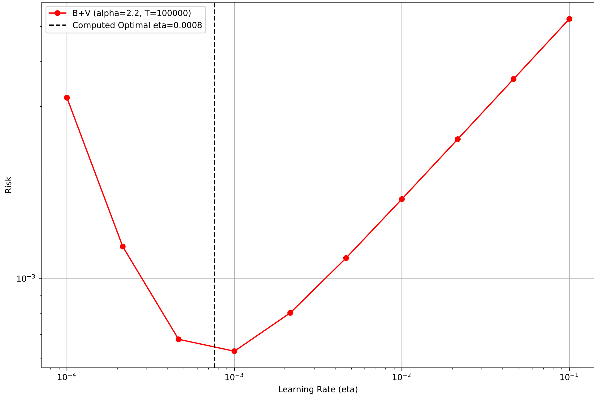
Risk for Different Learning Rates (SLOCK vs Diagonal) \alpha=2.2 , T=100000
