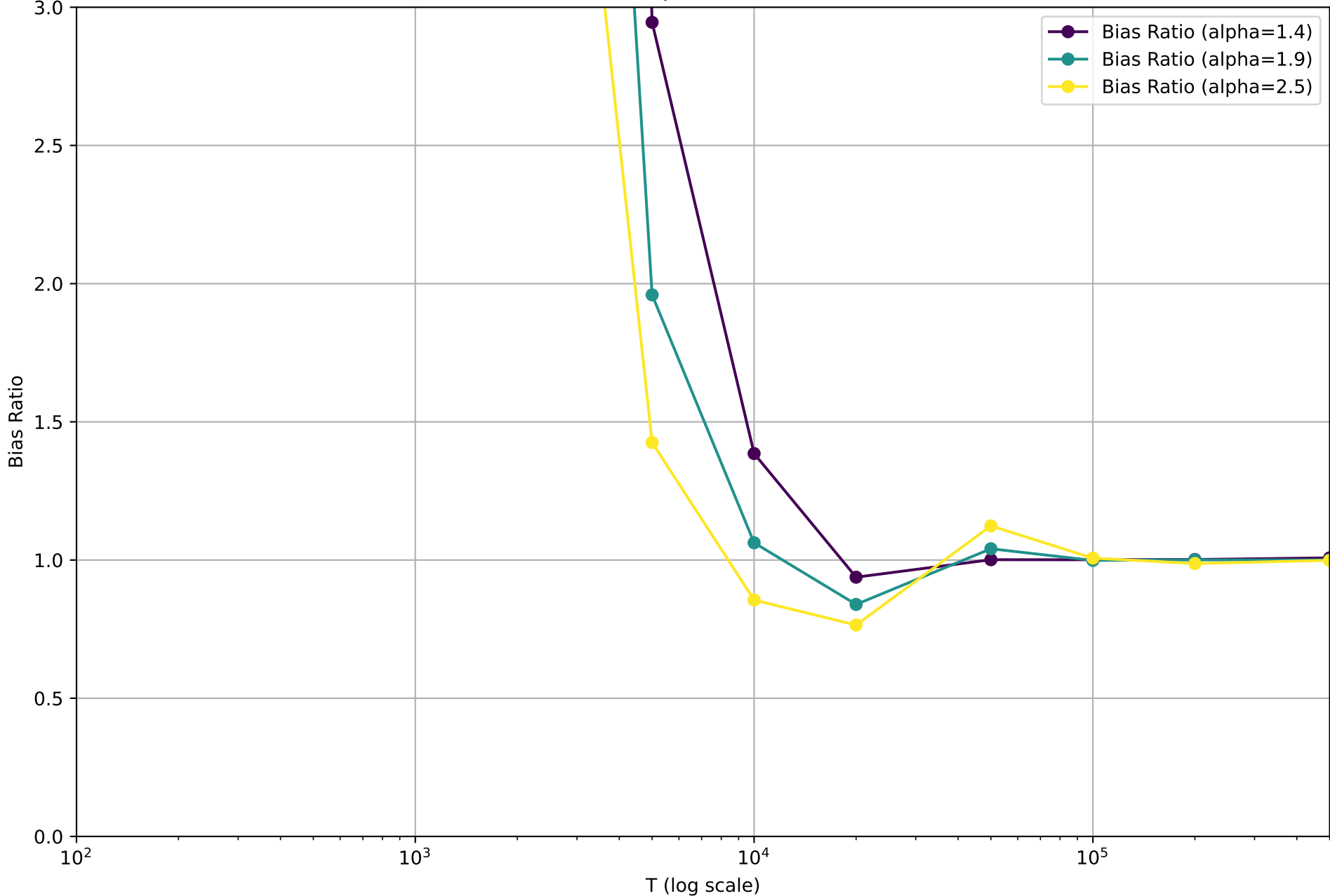
Bias Ratios for Different Alphas (slock vs True ) eta=0.0001
