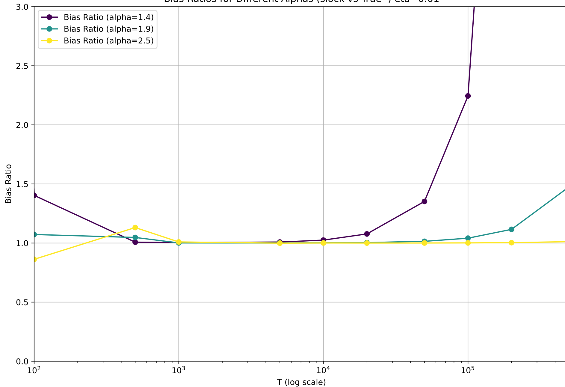
Bias Ratios for Different Alphas (slock vs True ) eta=0.01
