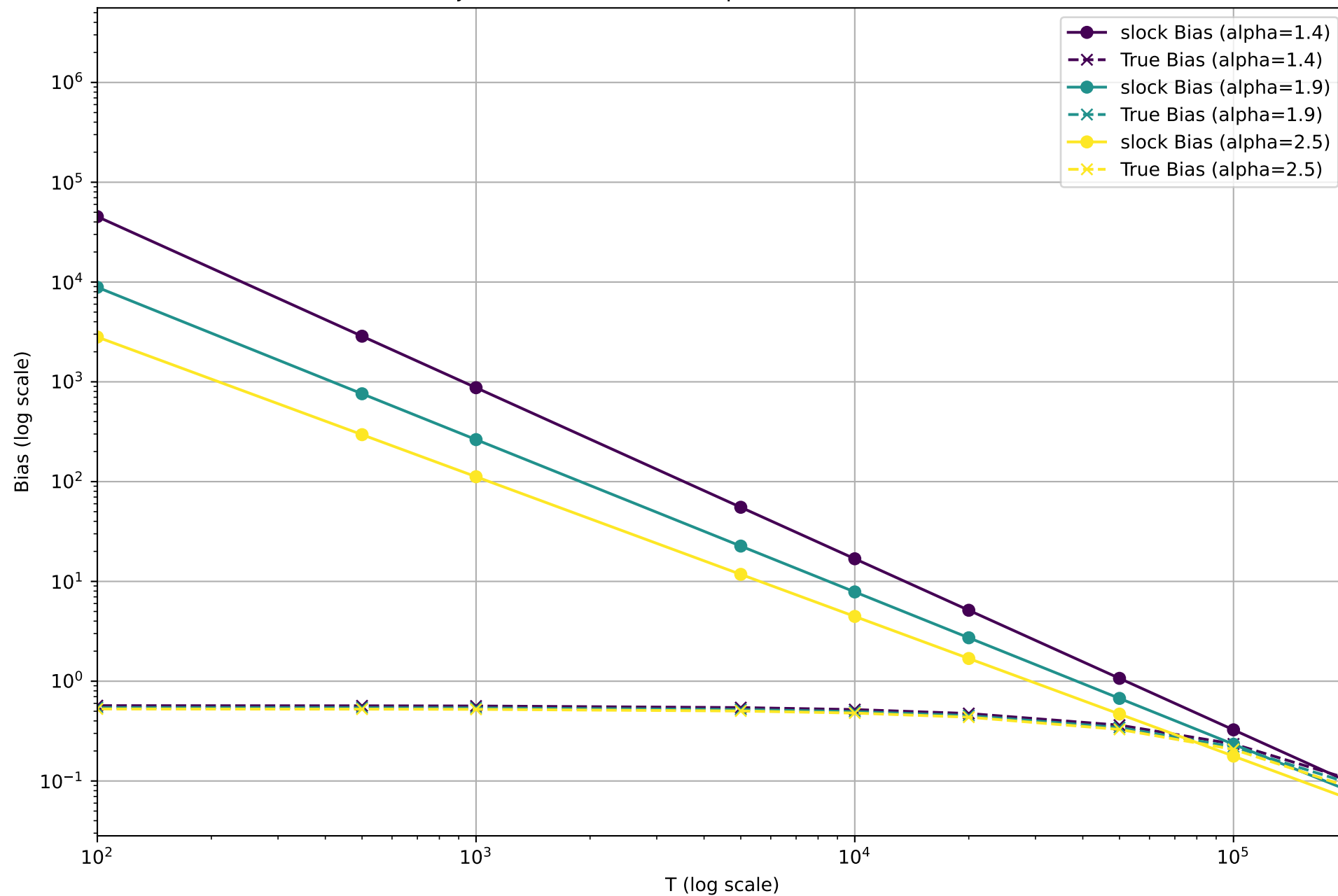
Bias Trajectories for Different Alphas (slock vs True) \eta=1e-05
