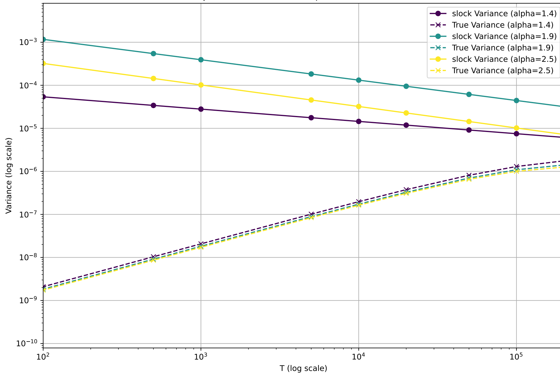
Variance Trajectories for Different Alphas (slock vs True) \eta=1e-05
