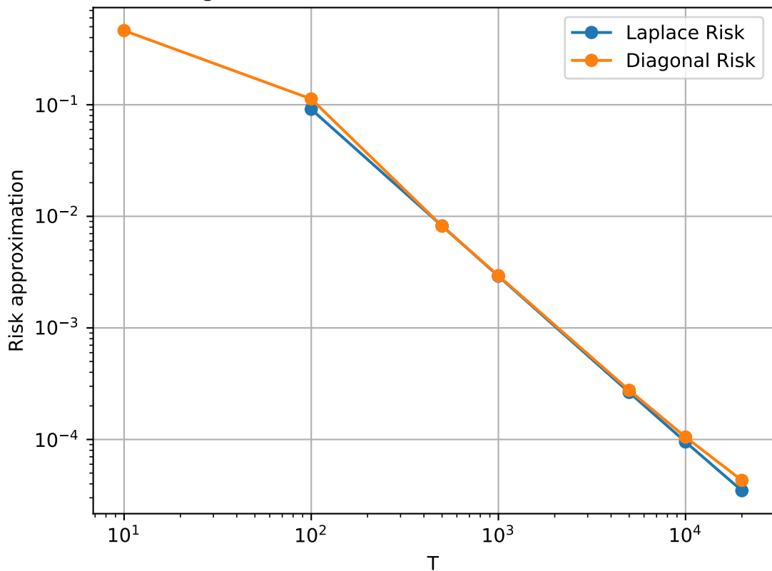
Total risk of Laplace approximation vs Diagonal approximation for wsd schedu sigma=0.1, beta=2, Tmax=20000, K=t/T=1
