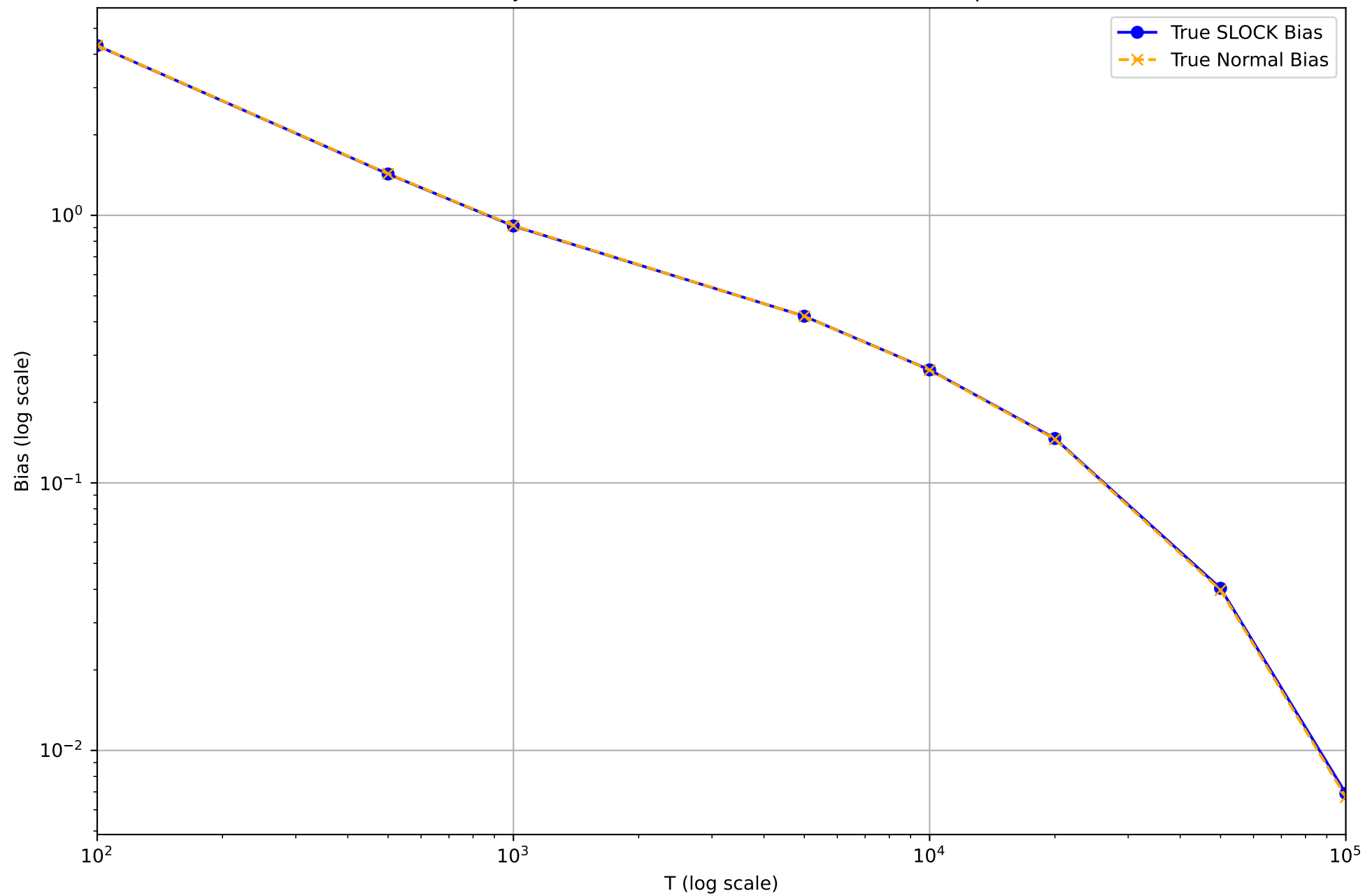
True Bias Trajectories (SLOCK vs Normal) \eta=0.01 , \alpha=1.3
