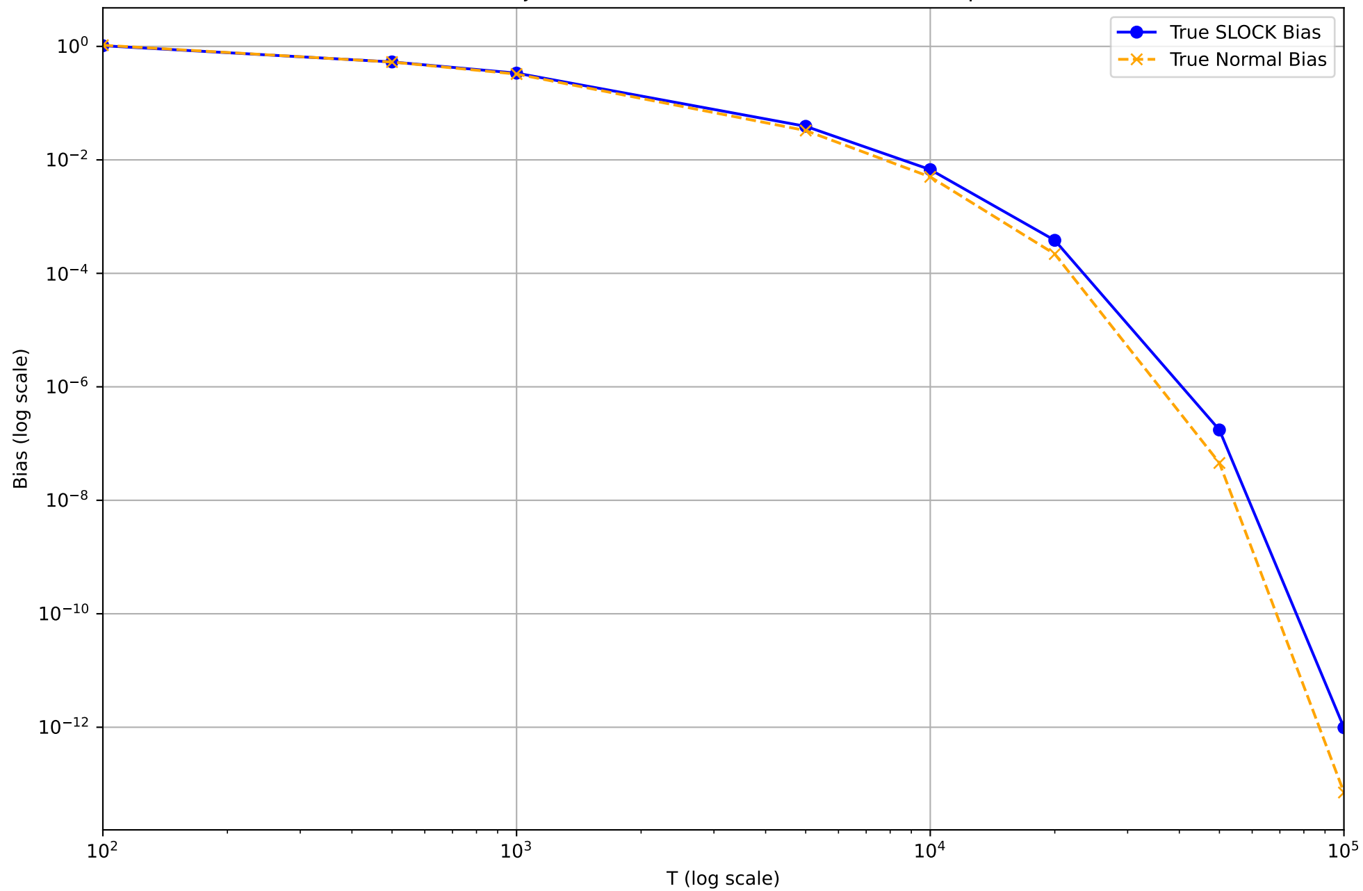
True Bias Trajectories (SLOCK vs Normal) \eta=0.1 , \alpha=1.3
