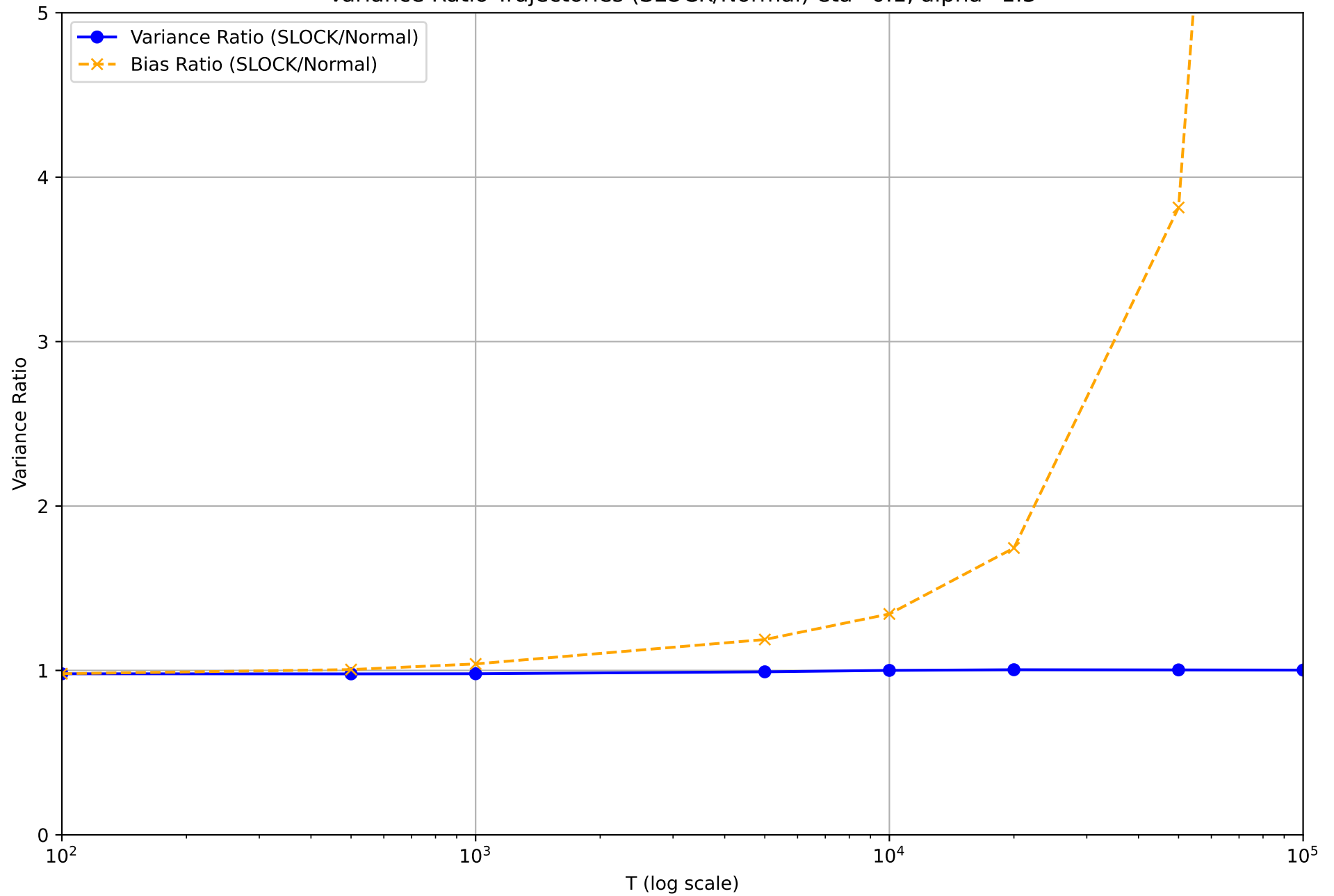
Variance Ratio Trajectories (SLOCK/Normal) \eta=0.1 , \alpha=1.3
