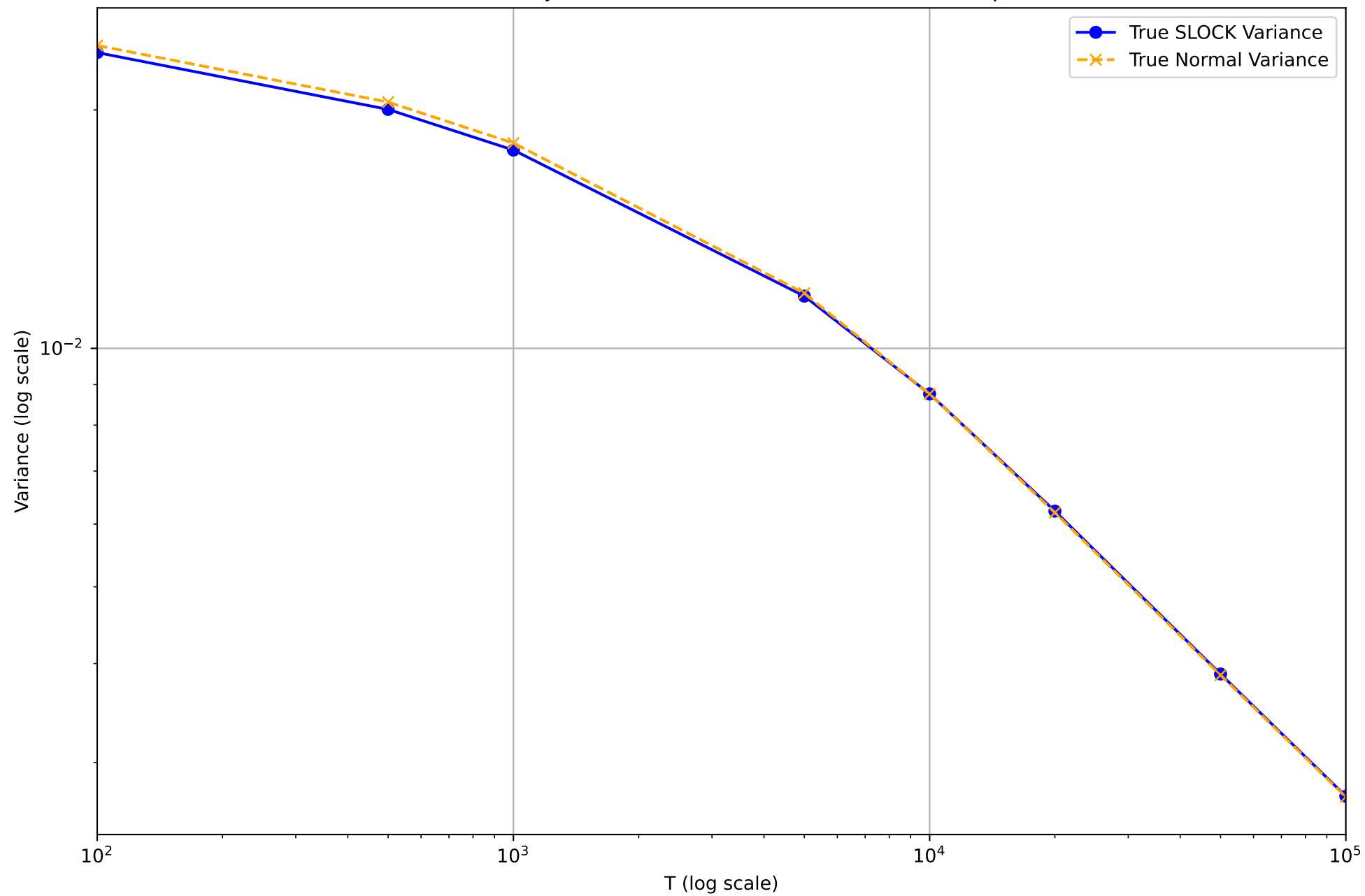
True Variance Trajectories (SLOCK vs Normal) \eta=0.1 , \alpha=1.3
