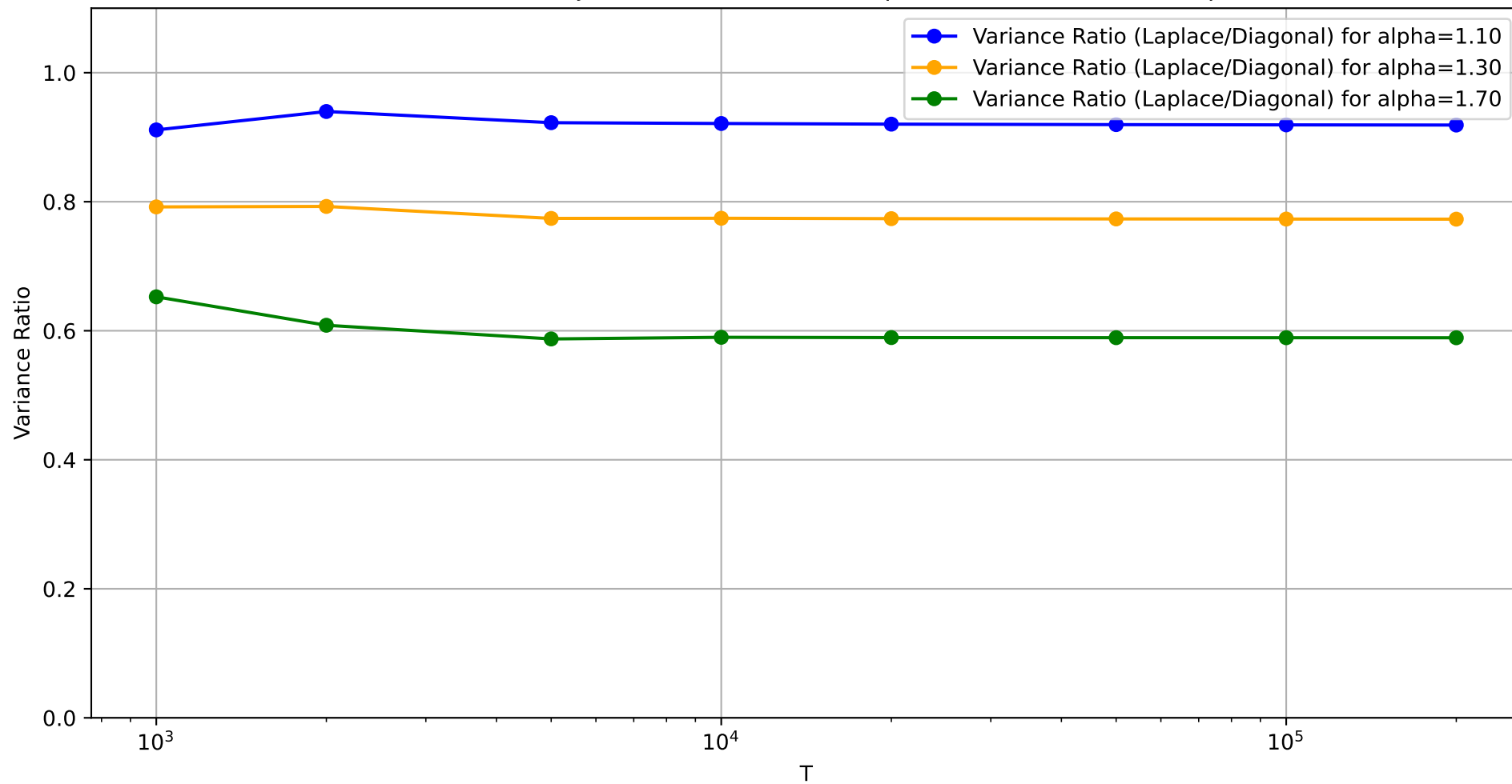
Variance Ratio Trajectories for Different Alphas, \text{dim}=(Tb50)^{**}(1b\alpha)
