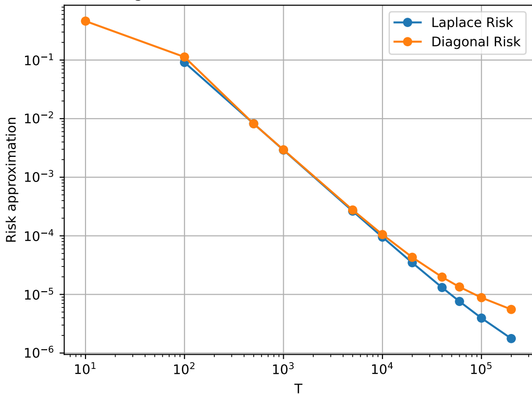
Total risk of Laplace approximation vs Diagonal approximation for wsd schedu sigma=0.1, beta=2, Tmax=200000, K=t/T=1
