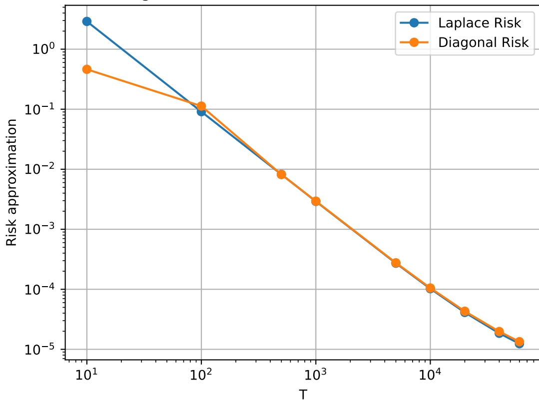
Total risk of Laplace approximation vs Diagonal approximation for wsd schedu sigma=0.1, beta=2, Tmax=60000, K=t/T=1
