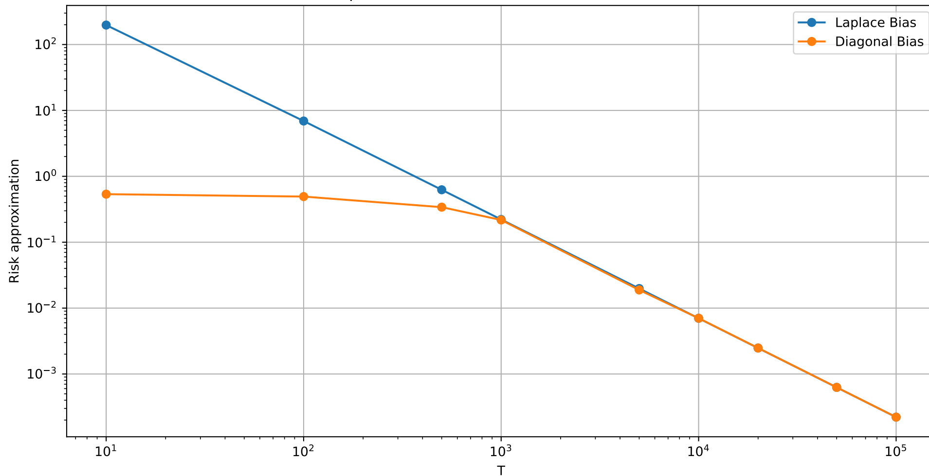
Bias components of Laplace approximation vs Diagonal approximation for linear schedule \alpha=2 , \beta=2 , T_{\max}=100000 , K=t/T=1
