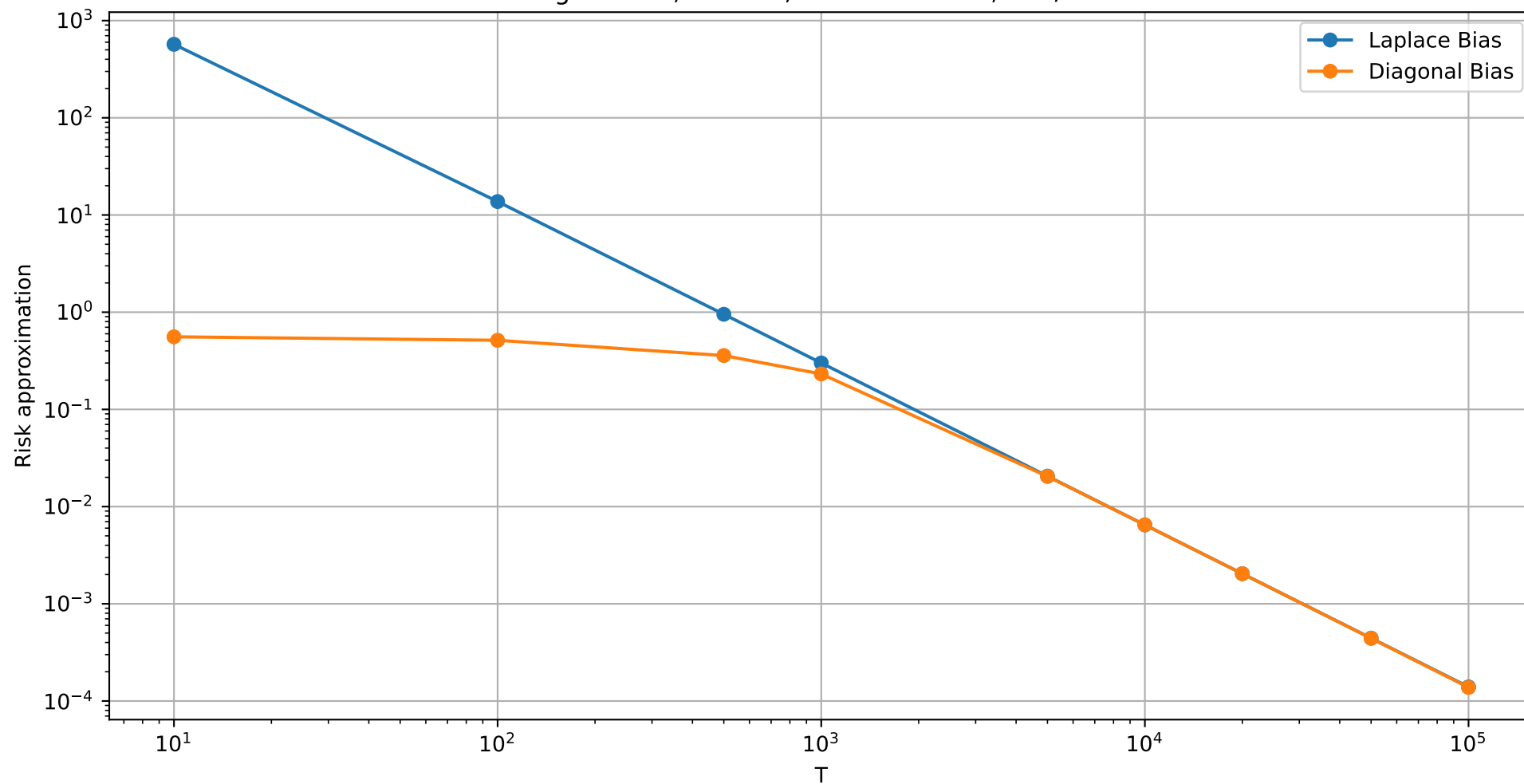
Bias components of Laplace approximation vs Diagonal approximation for linear schedule \sigma=0.5 , \beta=2 , T_{\max}=100000 , K=t/T=1
