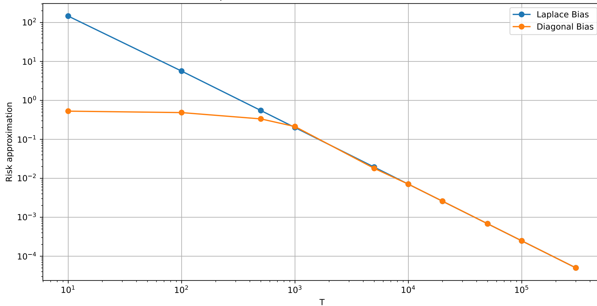
Bias components of Laplace approximation vs Diagonal approximation for linear schedule \alpha=2.2 , \beta=2 , T_{\max}=300000 , K=t/T=1
