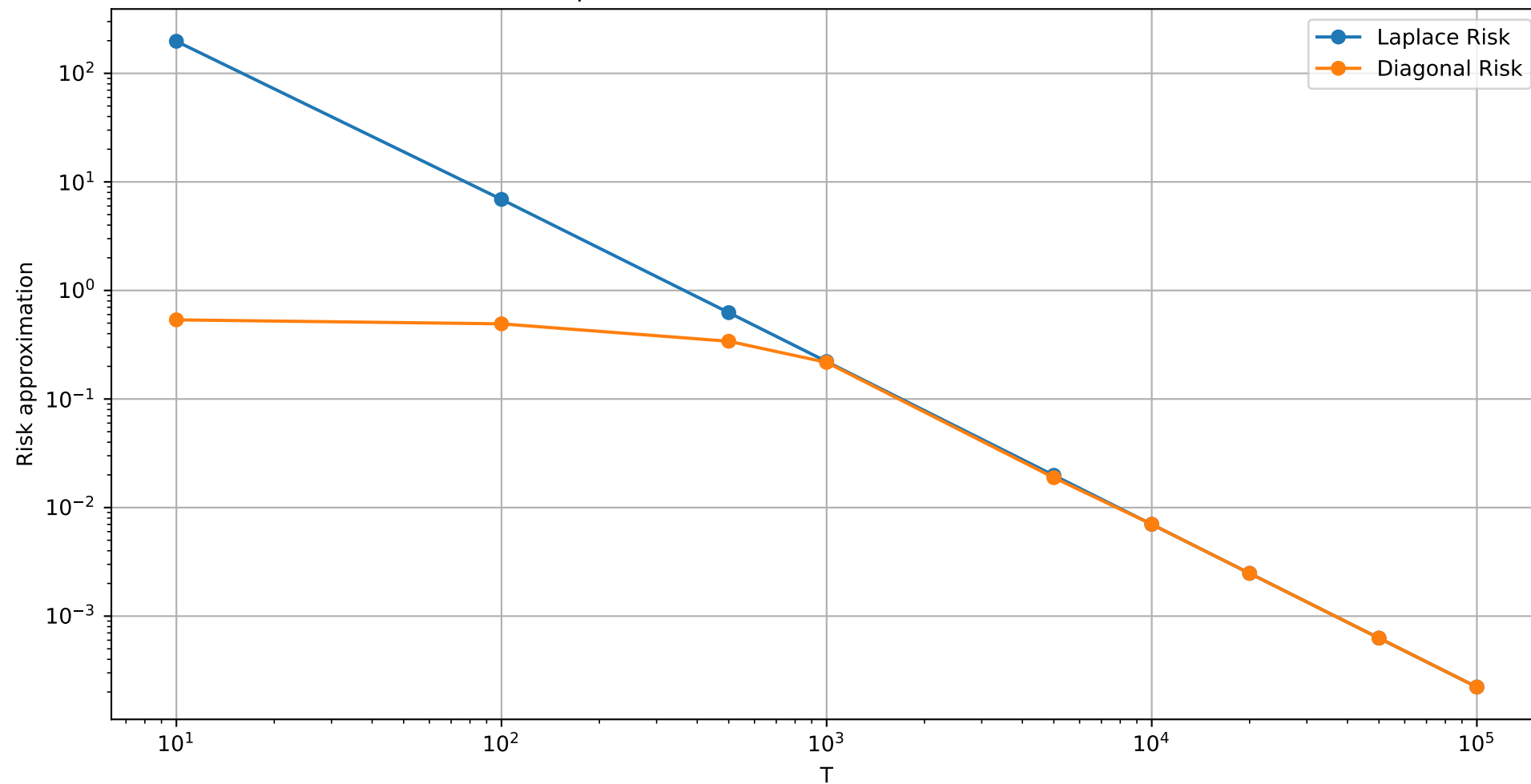
Total risk of Laplace approximation vs Diagonal approximation for linear schedule \alpha=2 , \beta=2 , T_{\max}=100000 , K=t/T=1
