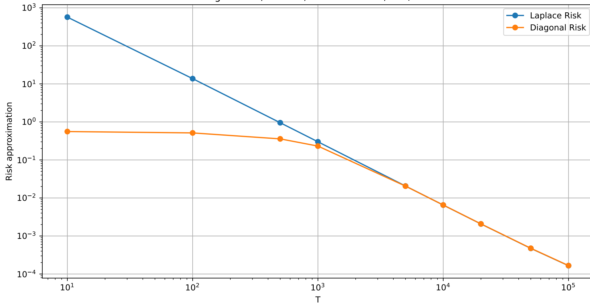
Total risk of Laplace approximation vs Diagonal approximation for linear schedule \sigma=0.5 , \beta=2 , T_{\max}=100000 , K=t/T=1
