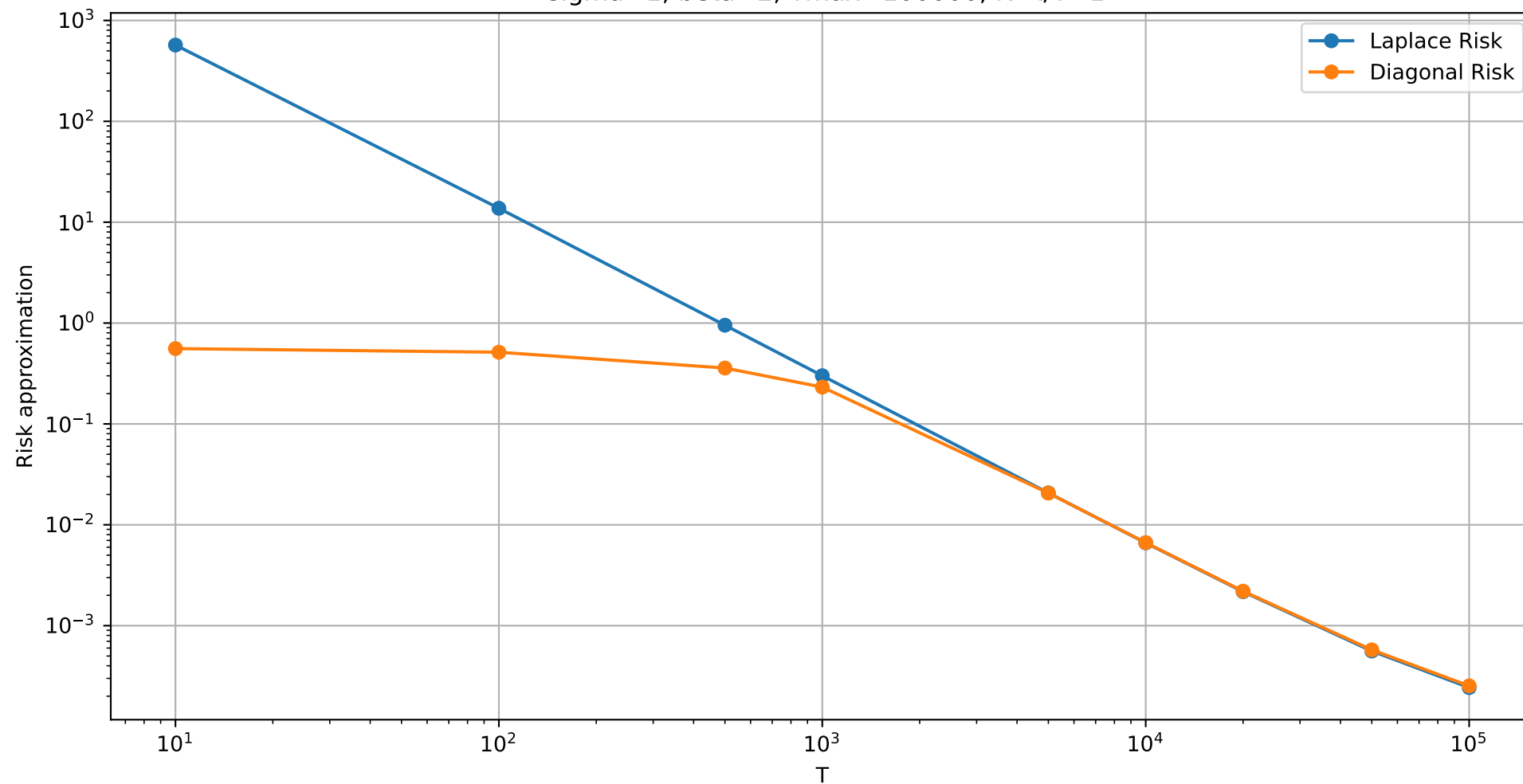
Total risk of Laplace approximation vs Diagonal approximation for linear schedule \sigma=1 , \beta=2 , T_{\max}=100000 , K=t/T=1
