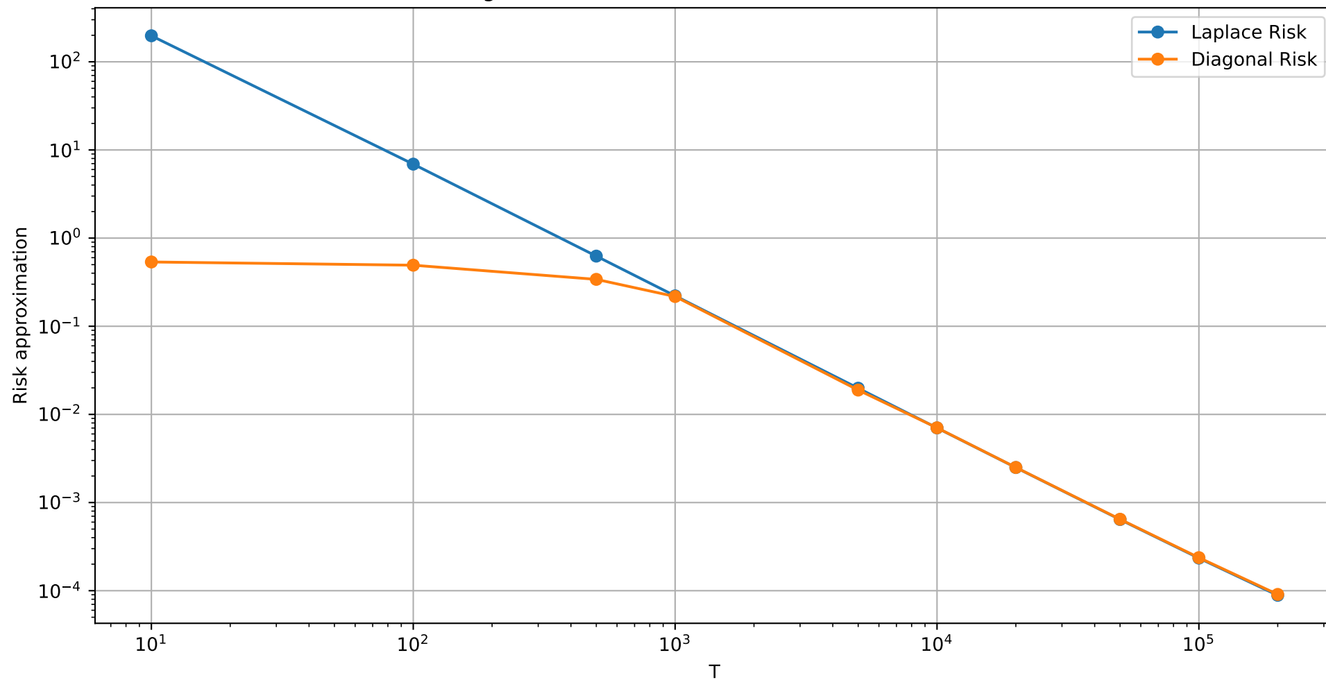
Total risk of Laplace approximation vs Diagonal approximation for linear schedule \sigma=0.5 , \beta=2 , T_{\max}=200000 , K=t/T=1
