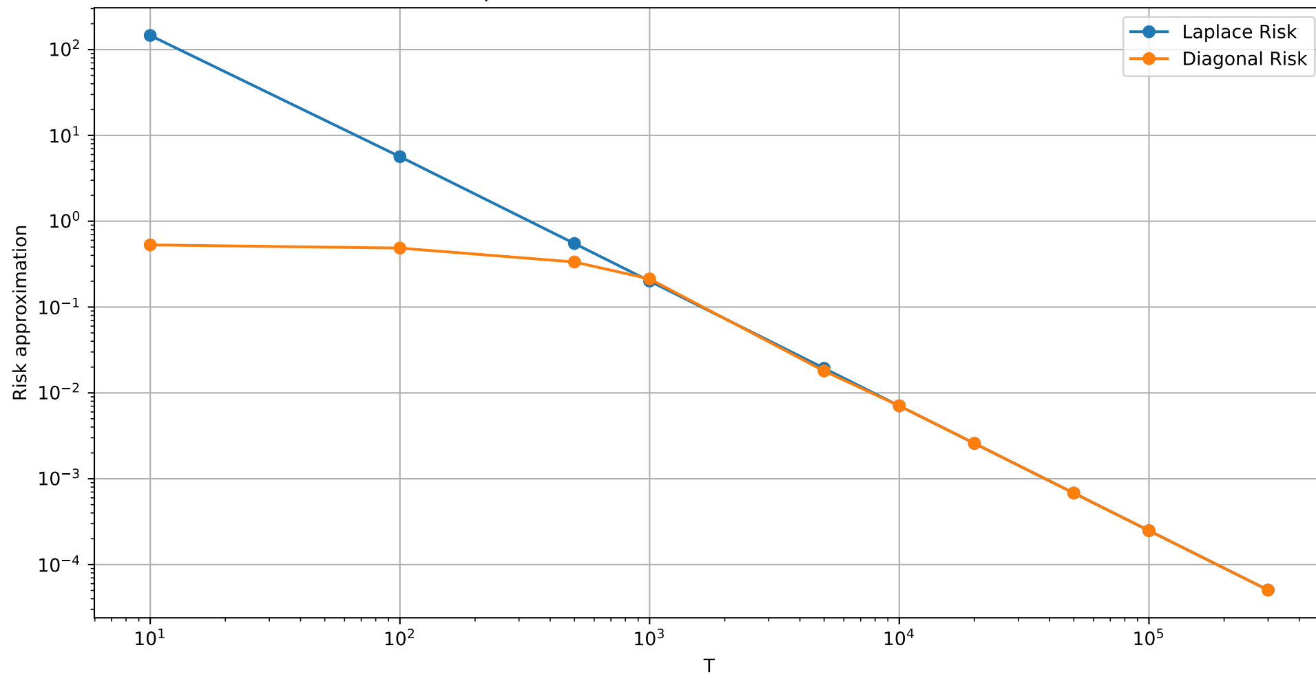
Total risk of Laplace approximation vs Diagonal approximation for linear schedule \alpha=2.2 , \beta=2 , T_{\max}=300000 , K=t/T=1
