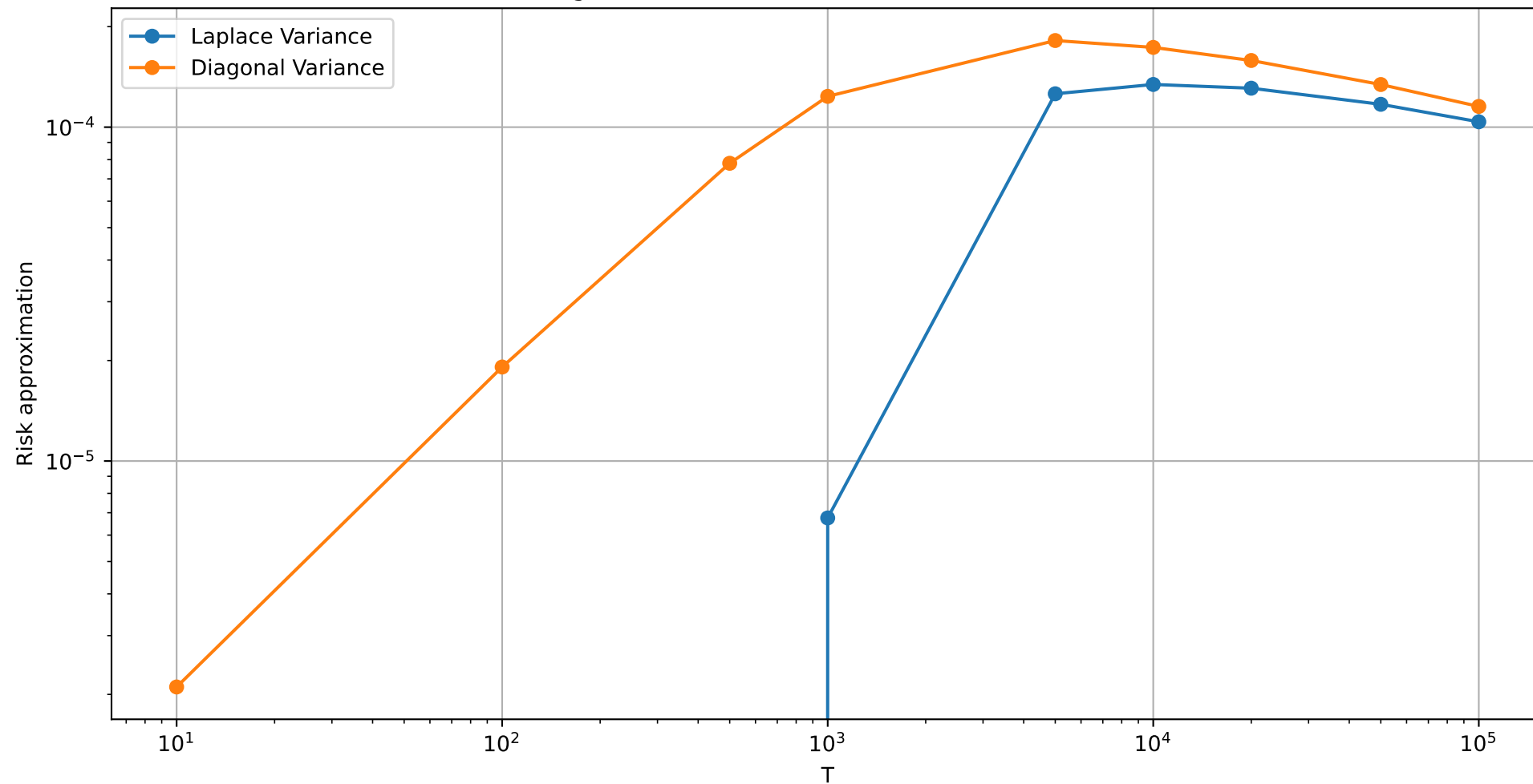
Variance components of Laplace approximation vs Diagonal approximation for linear schedule \sigma=1 , \beta=2 , T_{\max}=100000 , K=t/T=1
