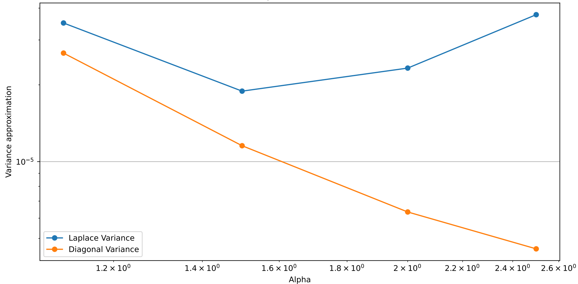
Variance of Laplace approximation vs Diagonal approximation for linear schedule at T=10000, K=1 for different alpha values, beta=2, Delta=1
