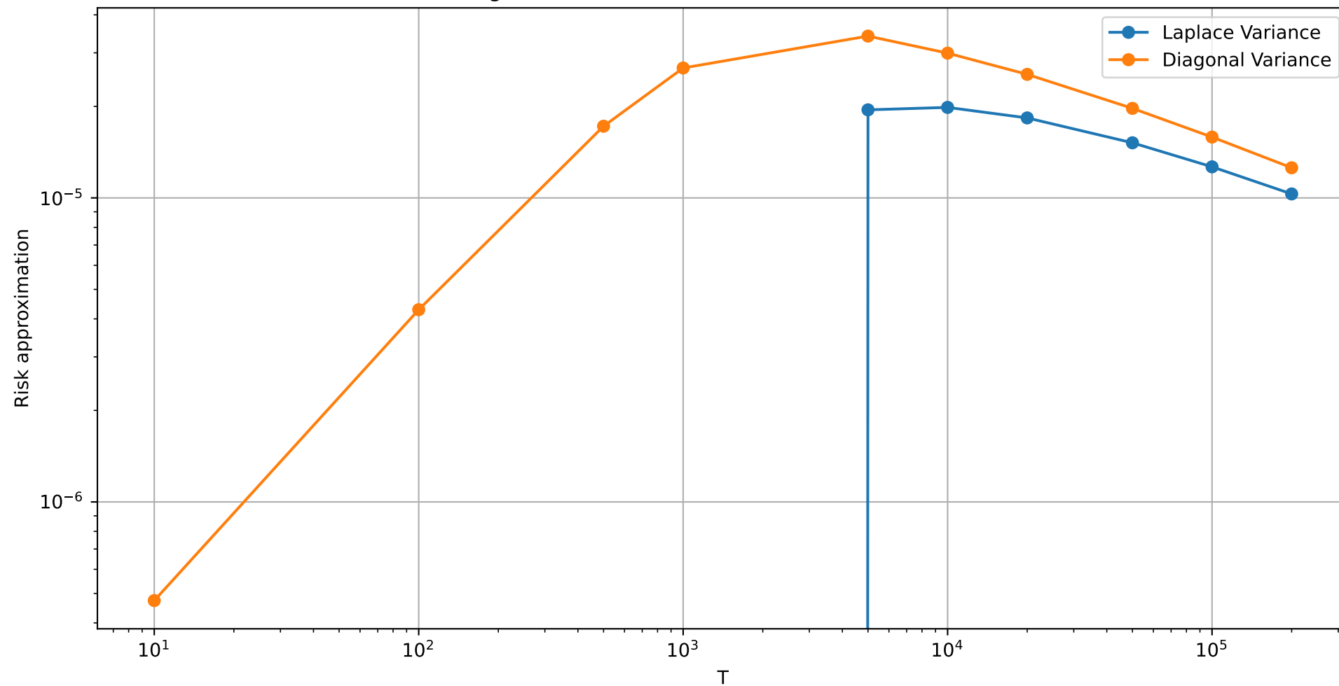
Variance components of Laplace approximation vs Diagonal approximation for linear schedule \sigma=0.5 , \beta=2 , T_{\max}=200000 , K=t/T=1
