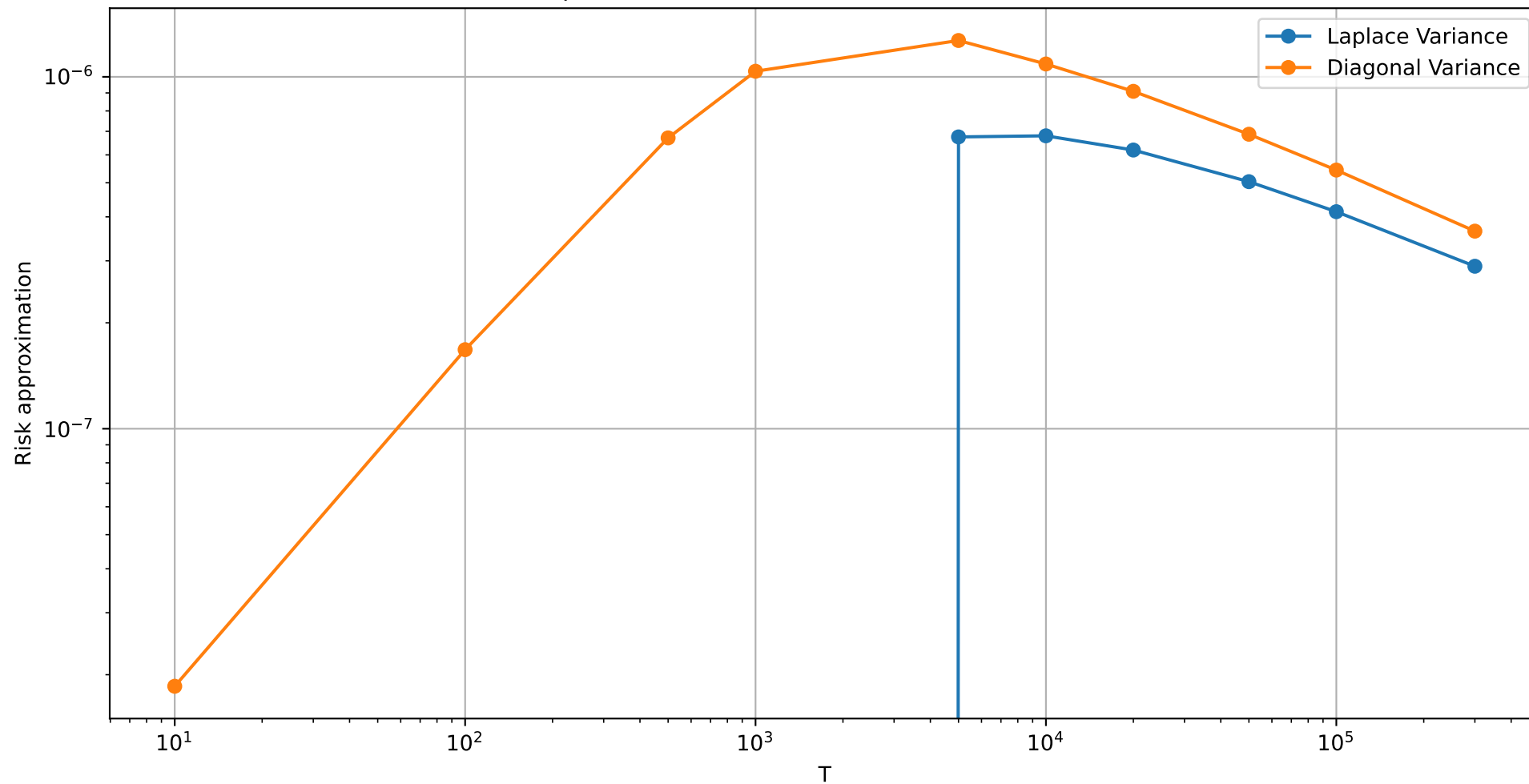
Variance components of Laplace approximation vs Diagonal approximation for linear schedule \alpha=2.2 , \beta=2 , T_{\max}=300000 , K=t/T=1
