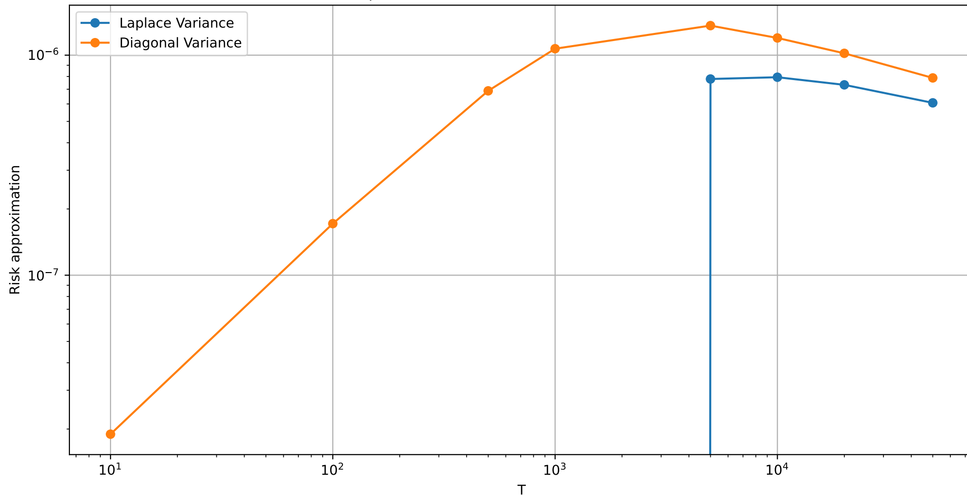
Variance components of Laplace approximation vs Diagonal approximation for linear schedule \alpha=2 , \beta=2 , T_{\max}=50000 , K=t/T=1
