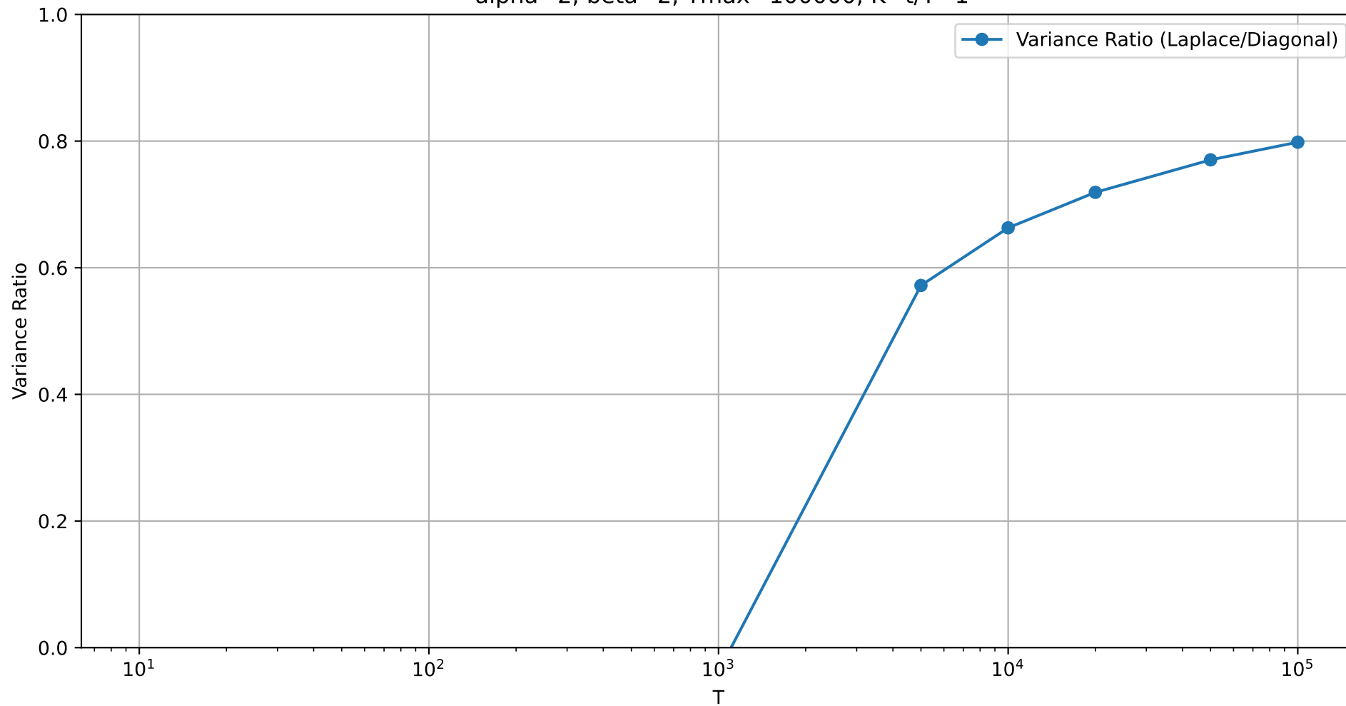
Variance Ratio of Laplace approximation to Diagonal approximation for linear schedule \alpha=2 , \beta=2 , T_{\max}=100000 , K=t/T=1
