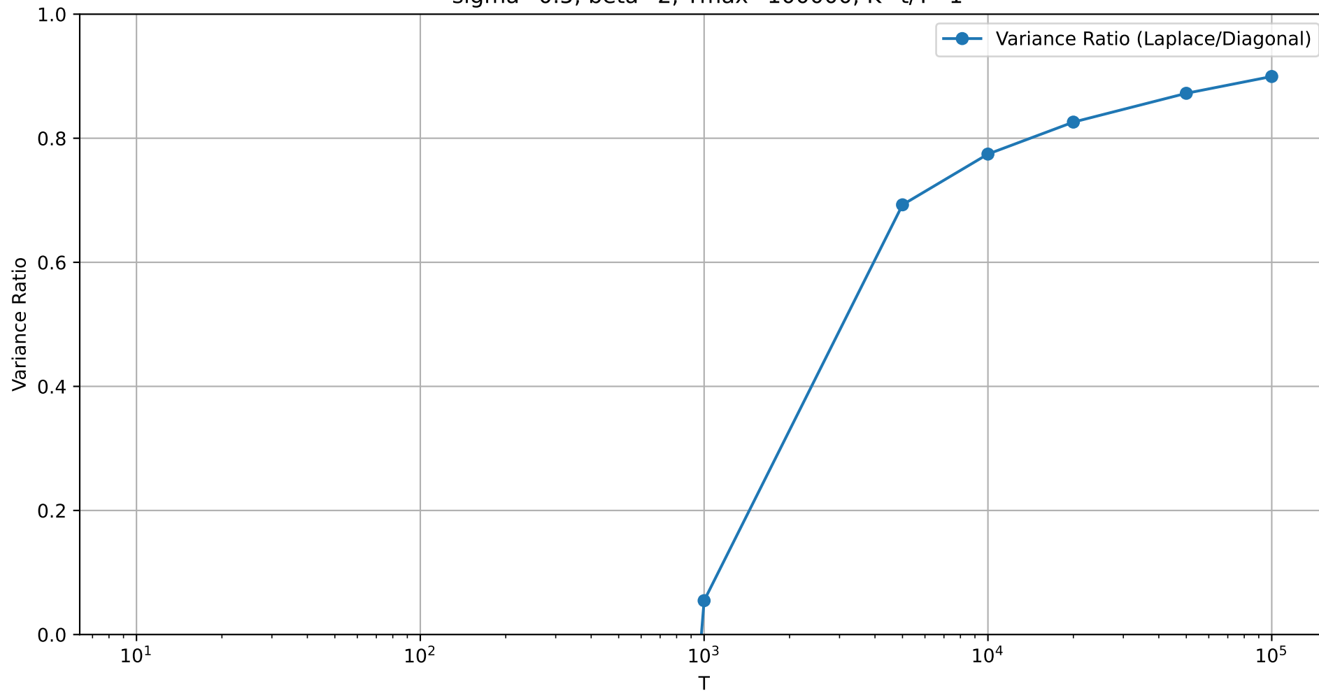
Variance Ratio of Laplace approximation to Diagonal approximation for linear schedule \sigma=0.5 , \beta=2 , T_{\max}=100000 , K=t/T=1
