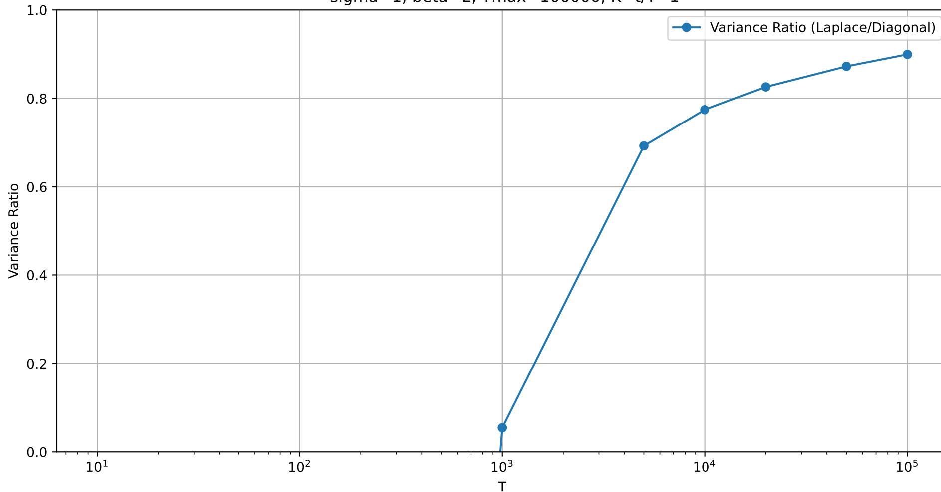
Variance Ratio of Laplace approximation to Diagonal approximation for linear schedule \sigma=1 , \beta=2 , T_{\max}=100000 , K=t/T=1
