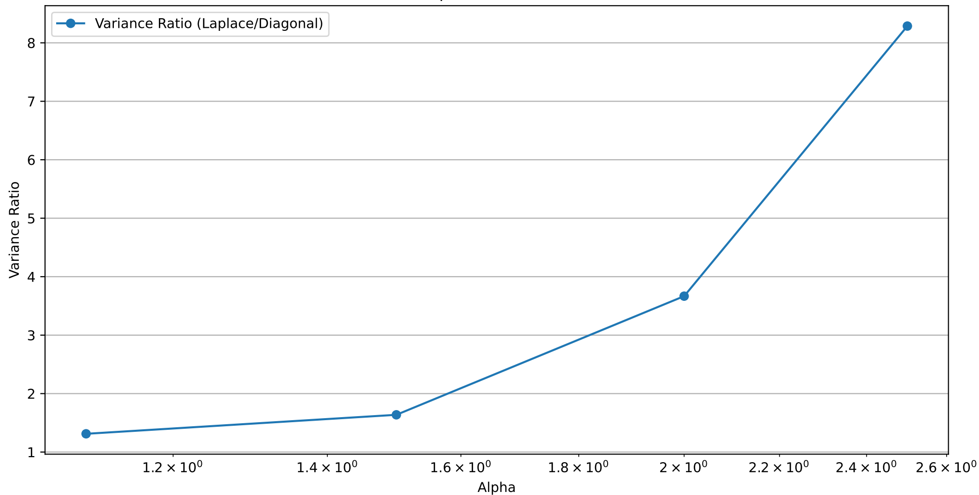
Variance Ratio of Laplace approximation to Diagonal approximation for linear schedule at T=10000 , K=1 for different alpha values, \beta=2 , \Delta=1
