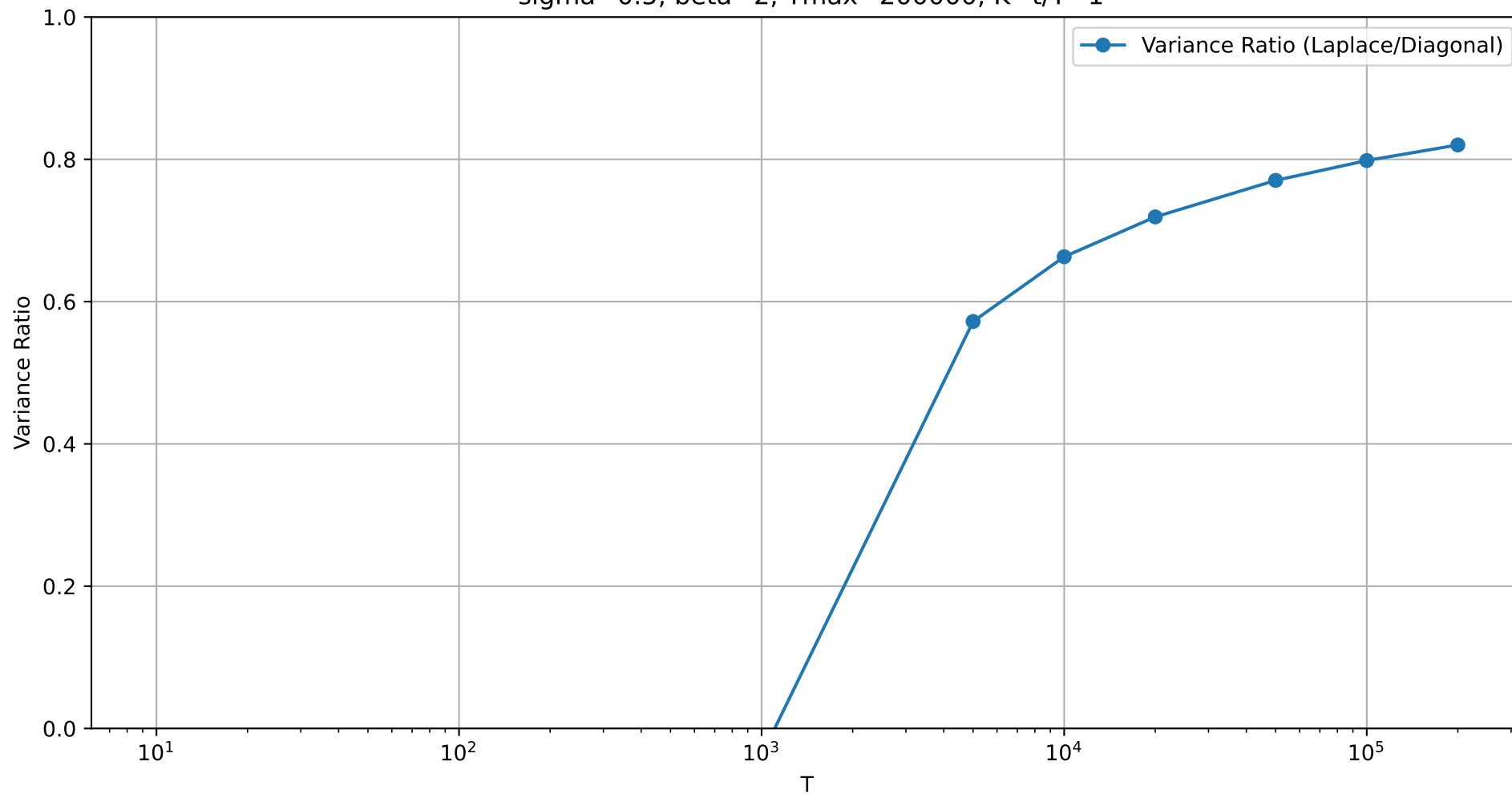
Variance Ratio of Laplace approximation to Diagonal approximation for linear schedule \sigma=0.5 , \beta=2 , T_{\max}=200000 , K=t/T=1
