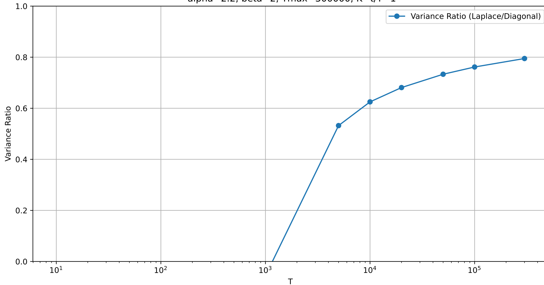
Variance Ratio of Laplace approximation to Diagonal approximation for linear schedule \alpha=2.2 , \beta=2 , T_{\max}=300000 , K=t/T=1
