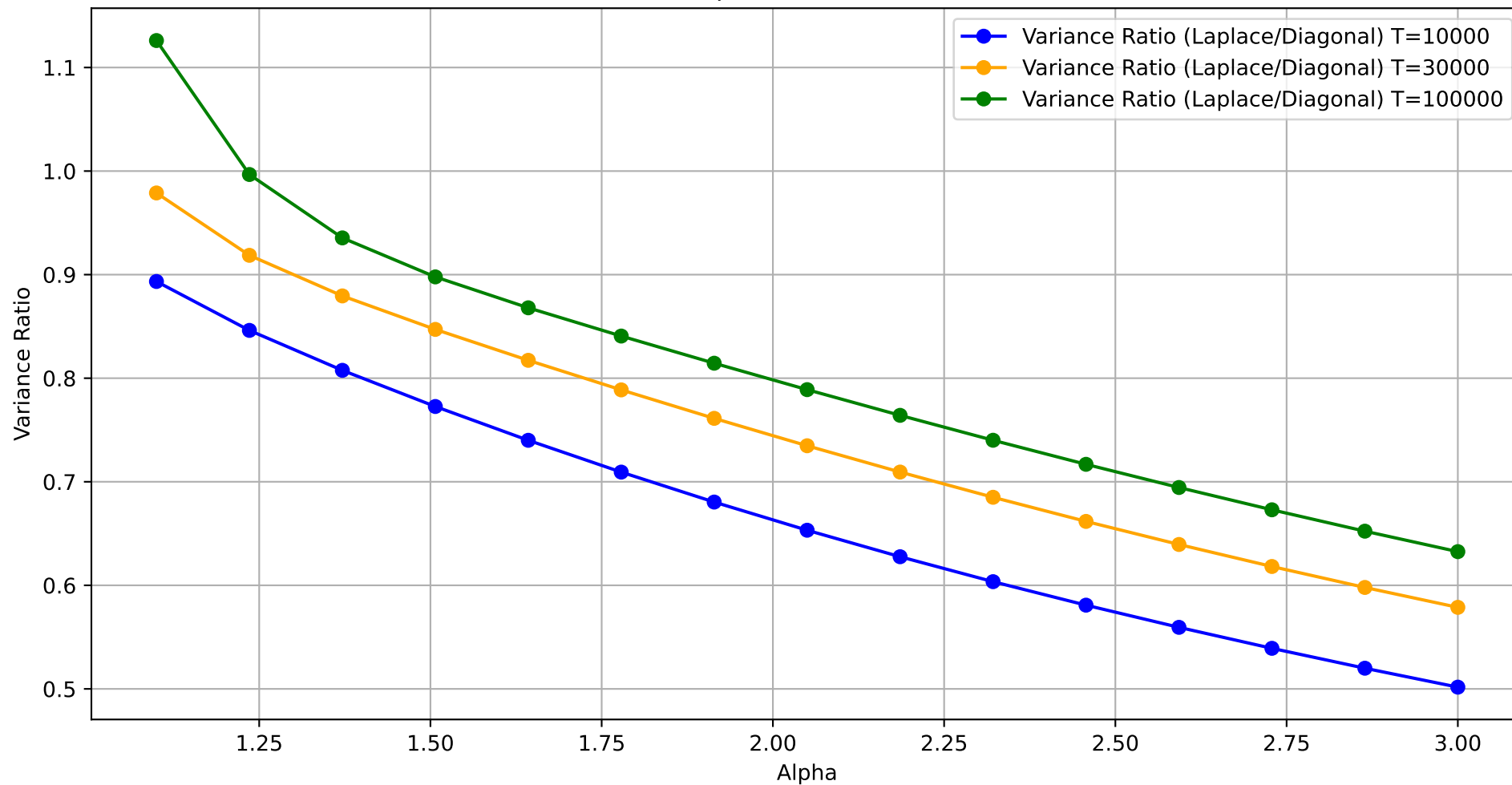
Variance Ratio of Laplace approximation to Diagonal approximation for linear schedule at K=1 for different alpha values, beta=2, Delta=1
