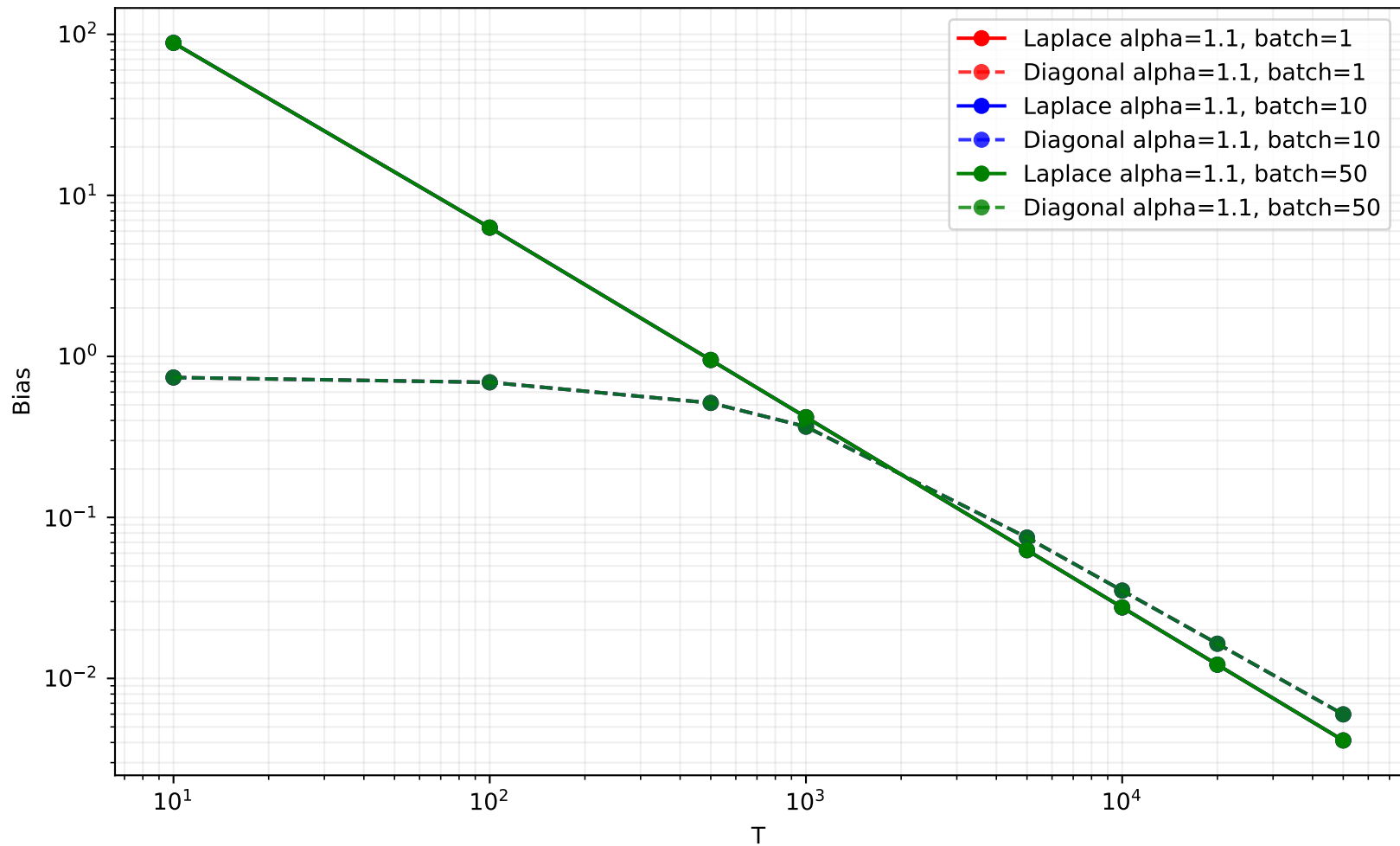
Bias trajectories for \alpha=1.1 and different batch sizes
