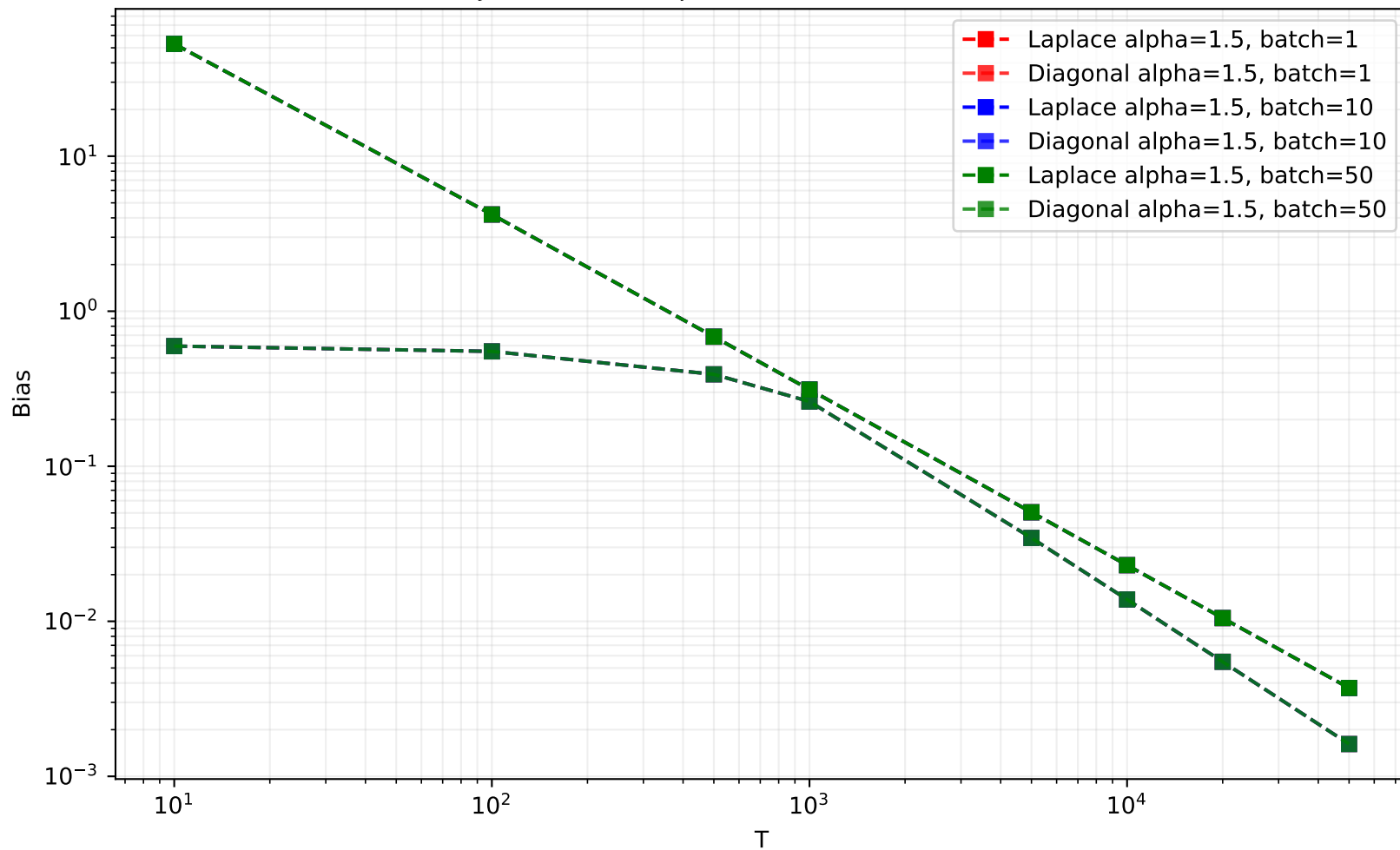
Bias trajectories for \alpha=1.5 and different batch sizes
